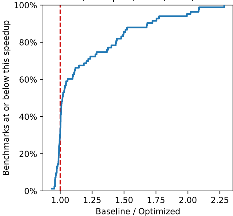
Empirical CDF of speedup (on Graphite/Vulkan, n=83)
