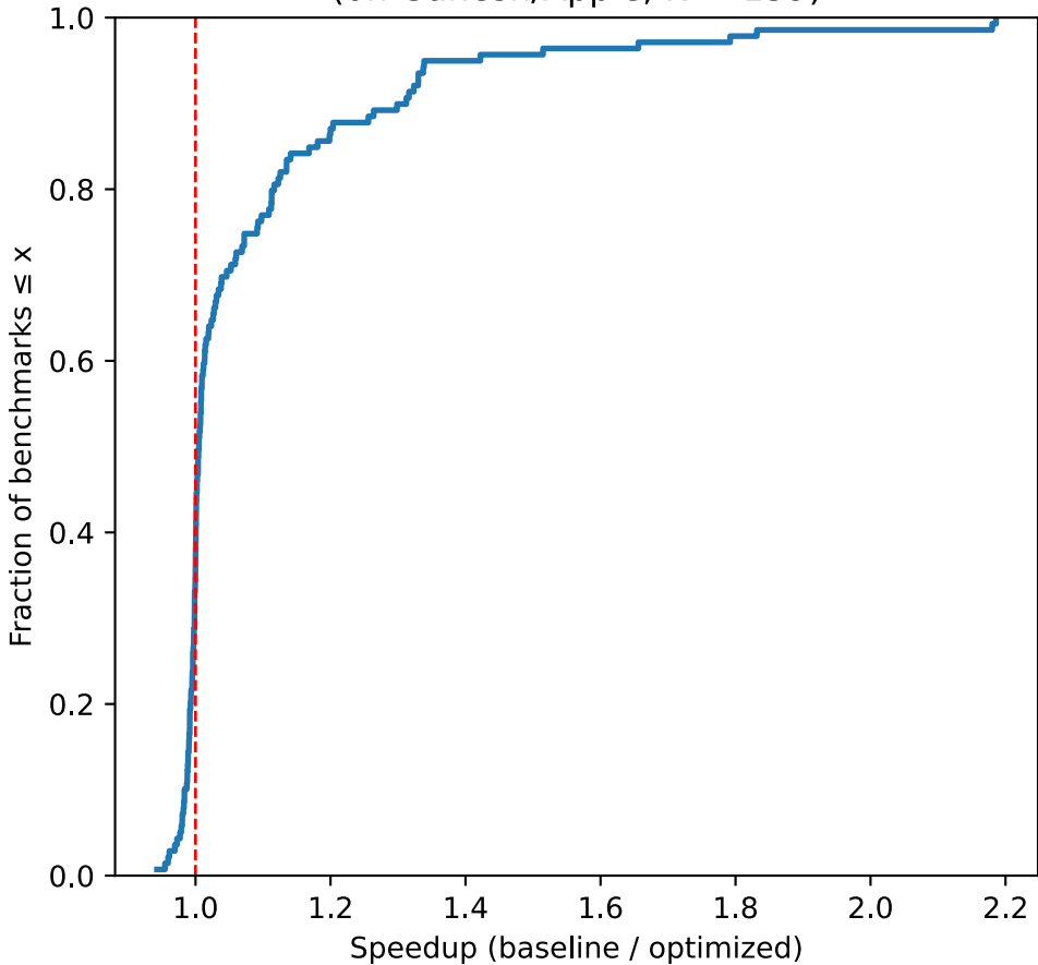
Empirical CDF of Speedup (on Ganesh/Apple, N = 139)
