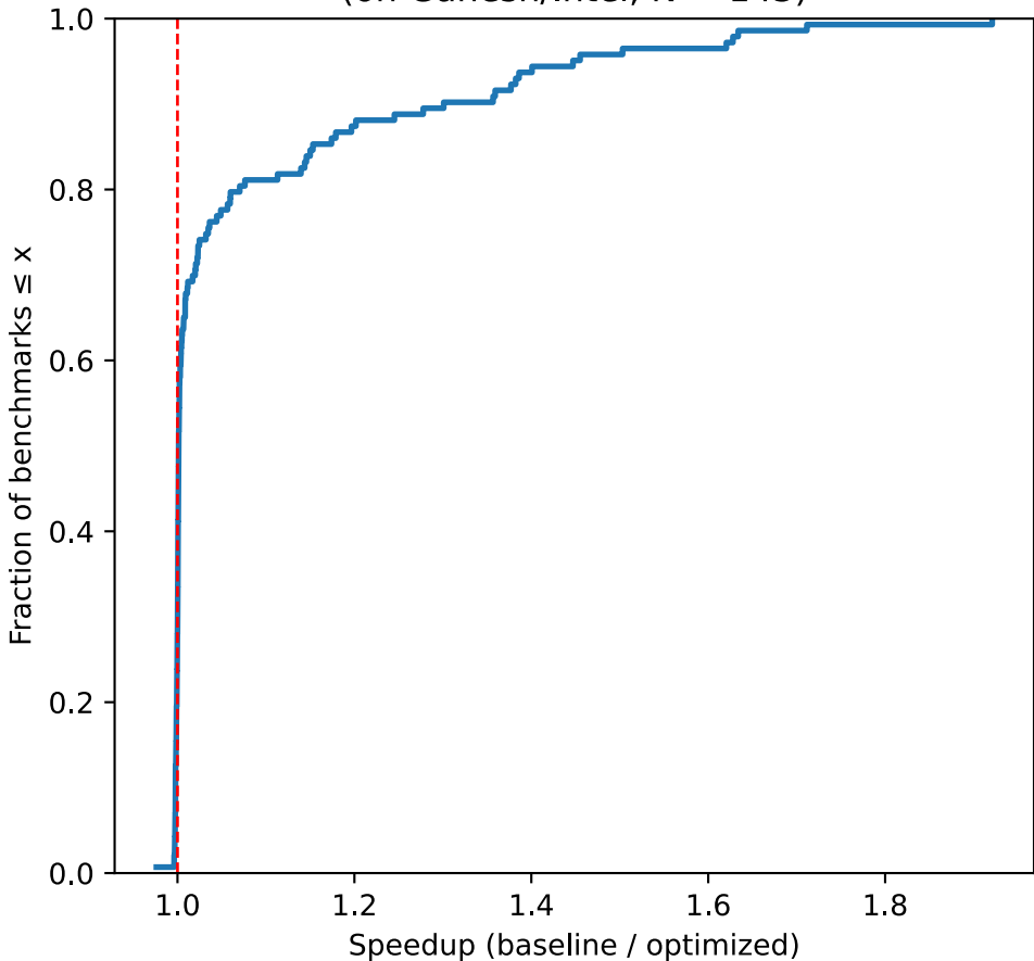
Empirical CDF of Speedup (on Ganesh/Intel, N = 143)
