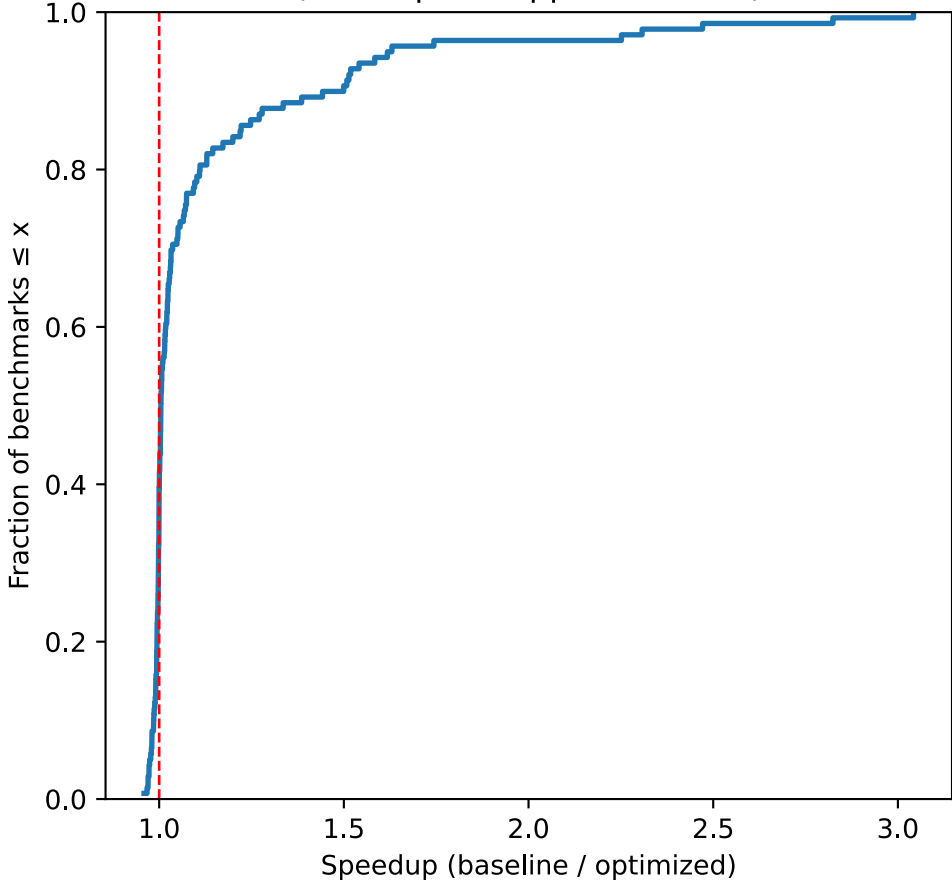
Empirical CDF of Speedup (on Graphite/Apple, N = 139)
