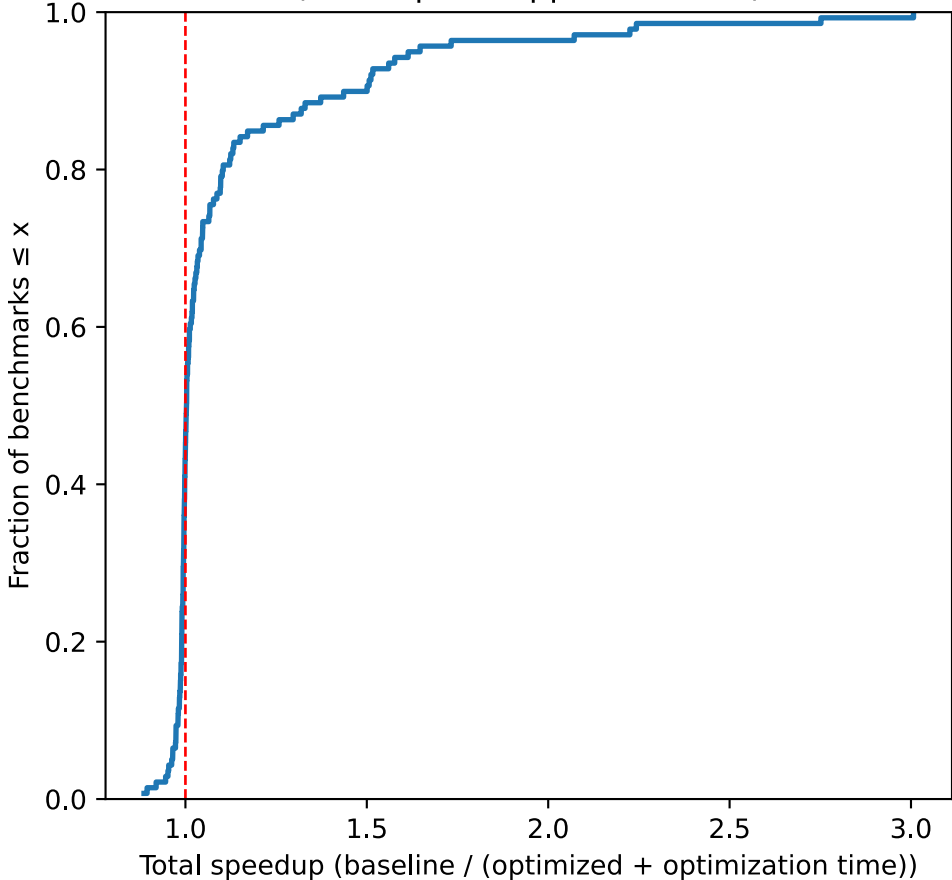
Empirical CDF of Total Speedup (on Graphite/Apple, N = 139)
