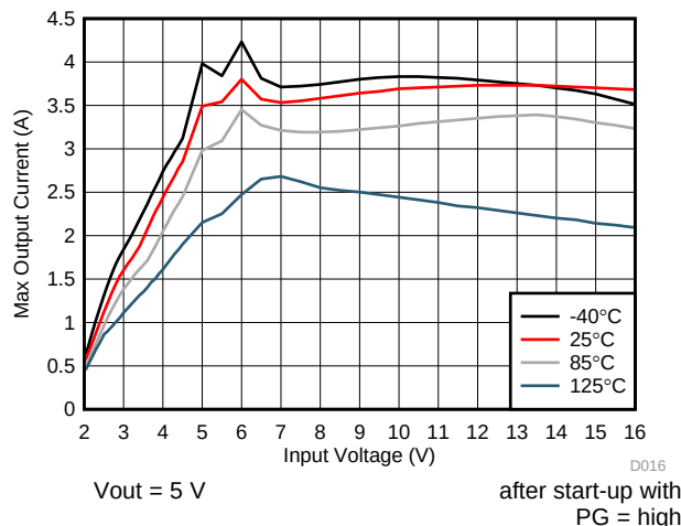
Figure 41. Maximum Load Current vs Input Voltage
