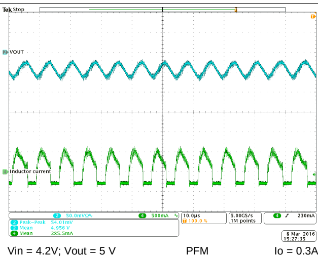
Figure 45. Output Voltage Ripple
