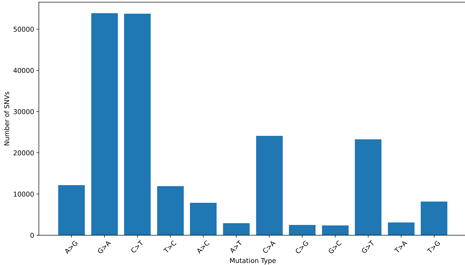
Somatic Mutation Spectrum
