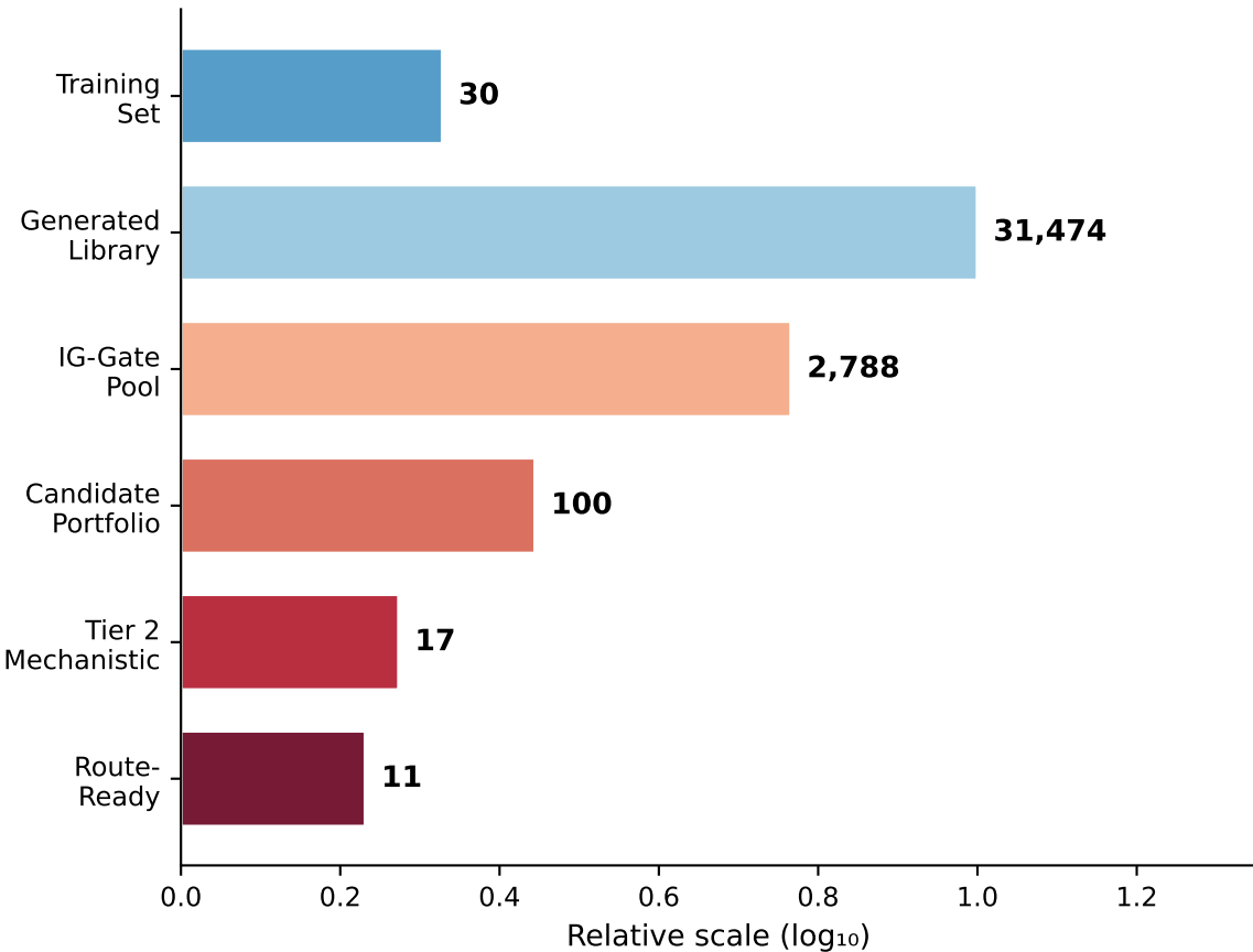
Hierarchical Selection Pipeline
