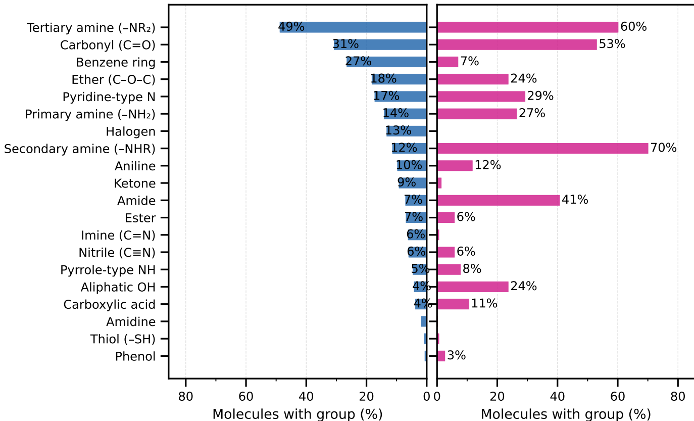
NIST Experimental (N = 1155 molecules)
