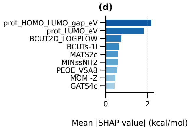
Feature importance — k-means
