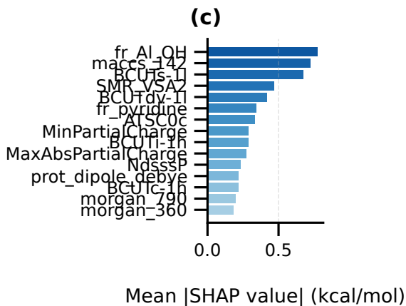
Feature importance — NIST
