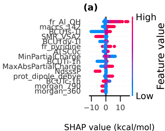
NIST — Molecular + PM7 features
