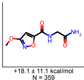
Amide
