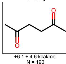
Carbonyl
