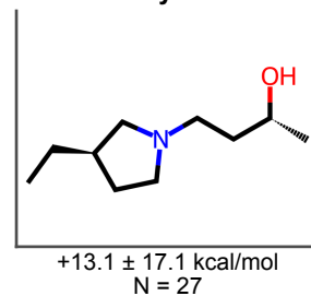
Tertiary amine
