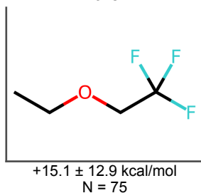
Ether
