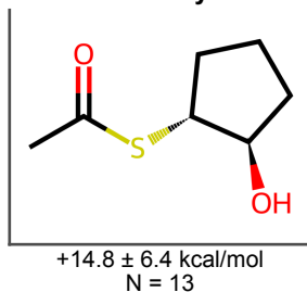
Carbonyl
