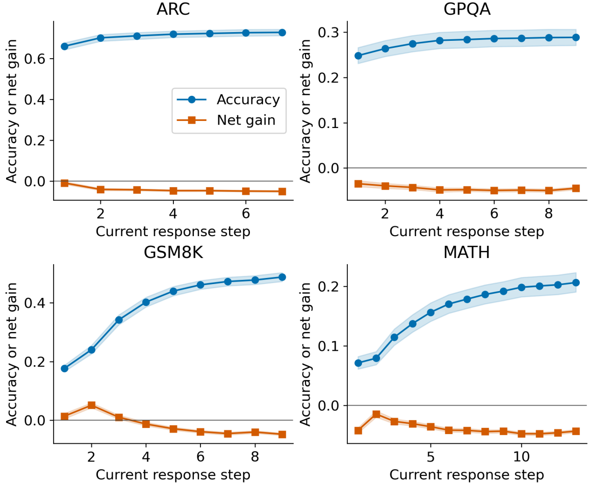
Figure 2. Population accuracy and continuation gain. Bands are task-cluster bootstrap intervals. The horizontal line marks zero net gain, not zero accuracy. Panel crossings do not identify an optimal action for every prefix.
