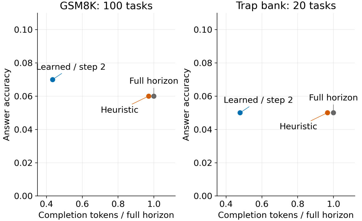
Figure 3. Actual paired answer quality and completion cost. Learned points stop at two on every task and provide no demonstrated adaptation beyond that fixed budget. Point estimates omit intervals, reported in Table 3.
