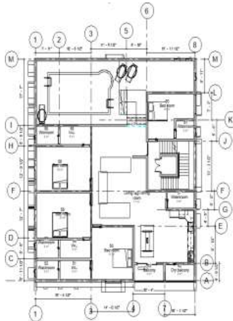
Fig.(5) Third Floor Plan Third Floor – 3329.78 SF
