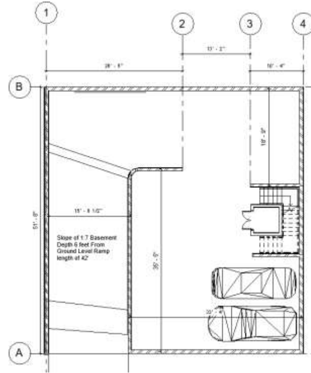
Fig.(1) Basement Floor Plan
