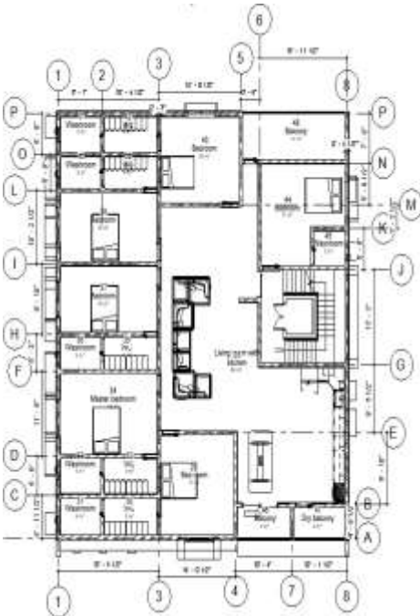
Fig.(4) Second Floor Plan Second Floor – 3345.28 SF
