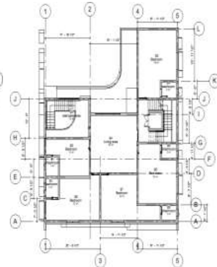
Fig.(7) Fifth Floor Plan Fifth Floor – 2798.78 SF
