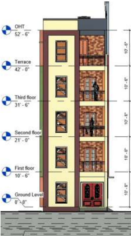
Fig.(6) Front Elevation
