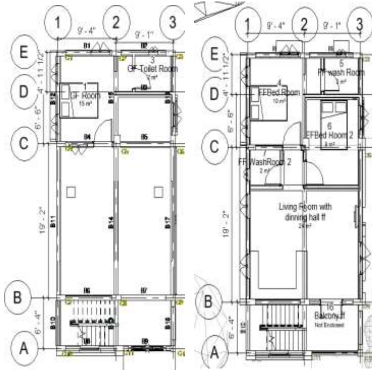
Fig.(1) Ground Floor Plan
