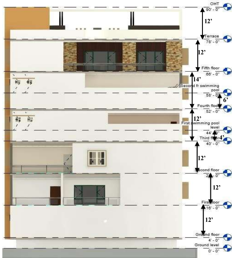
Fig.(10) Front Elevation
