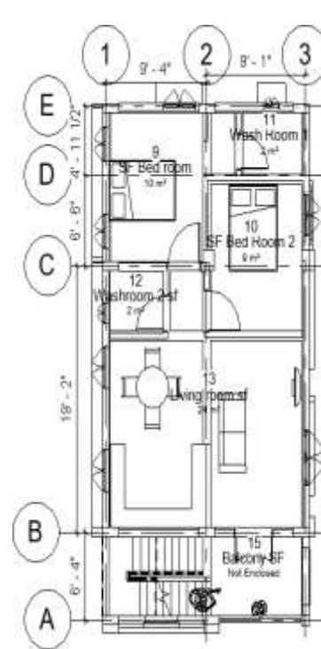
Fig.(3) Second Floor Plan
