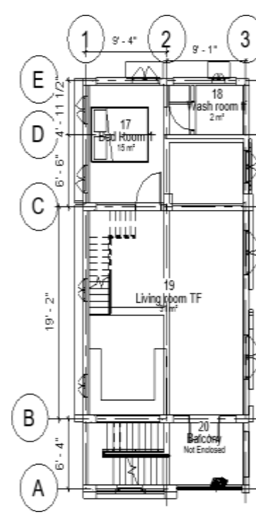
Fig.(4) Third Floor Plan
