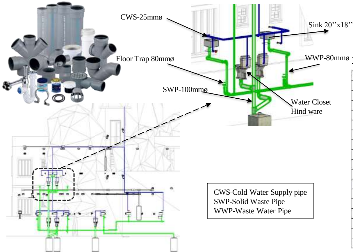
Fig.(11) Plumbing section
