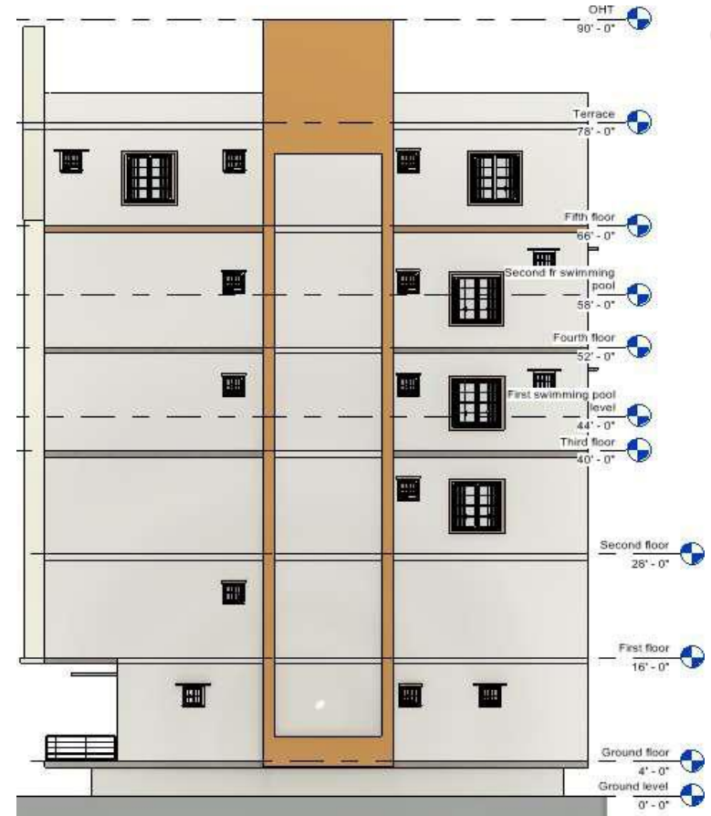
Fig.(11) Side Elevation
