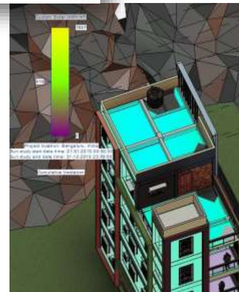
Solar Analysis Model
