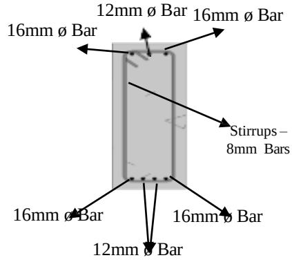
Beam Section:
