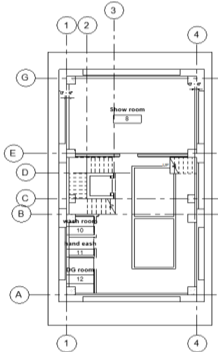
Fig.(1) Basement Floor Plan
