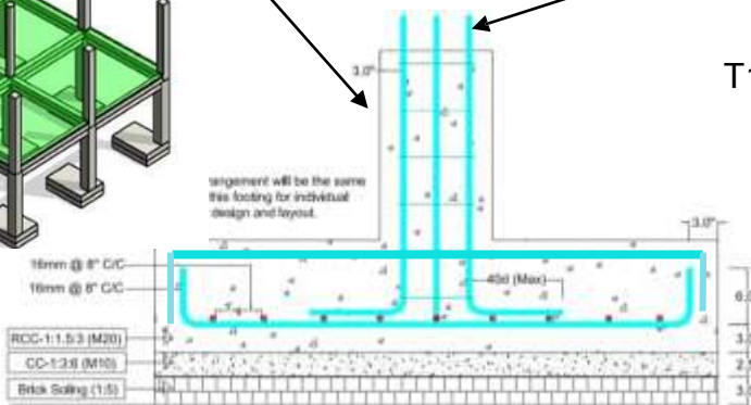
Foundation/Footing Detailing
