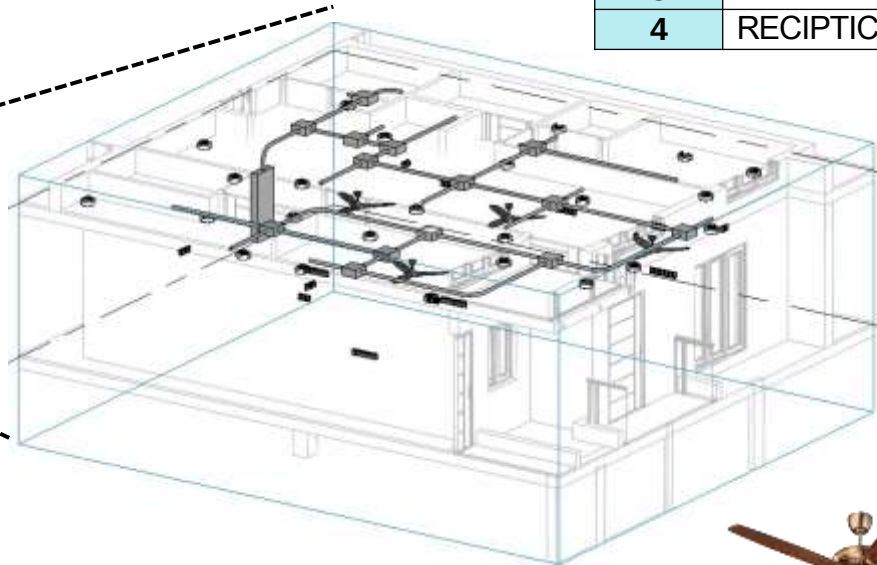
3D - ELECTRICAL
