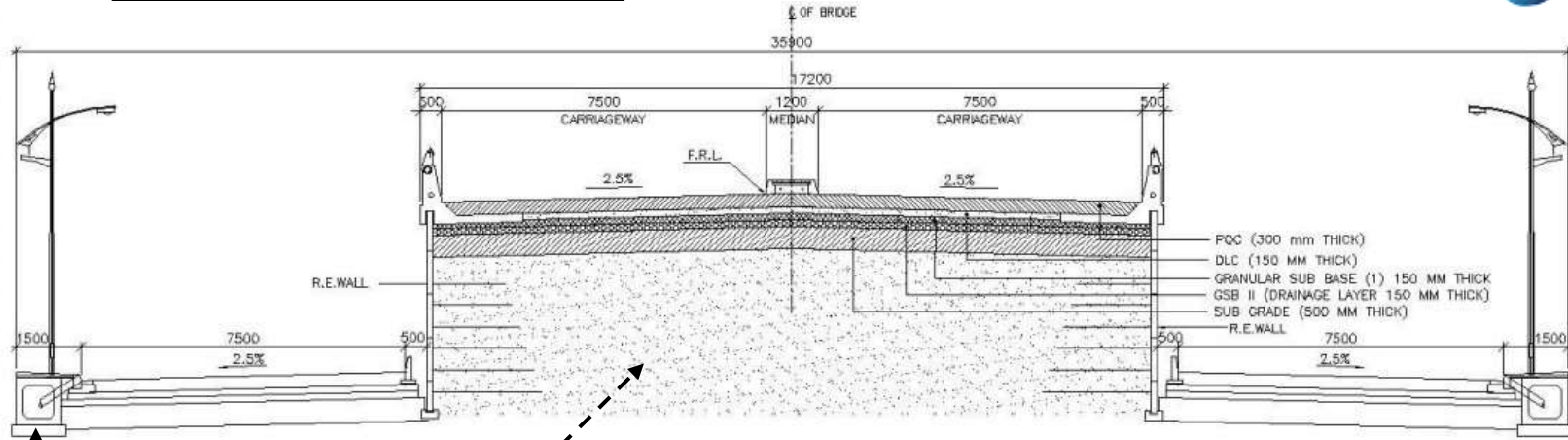
CROSS SECTION (SCALE-1:100)
