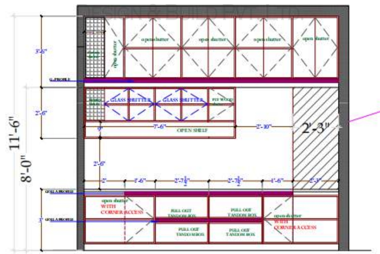
SOUTH WALL
