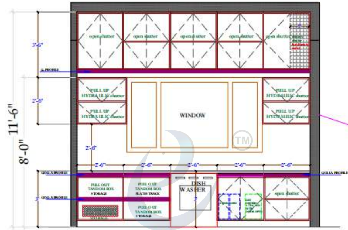
NORTH WALL
