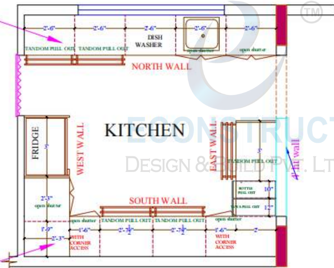
KITCHEN PLAN
