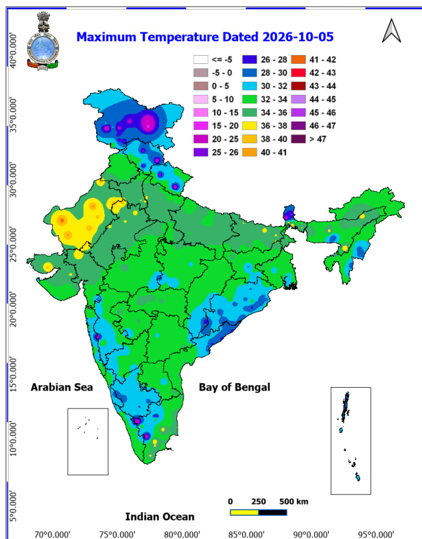
Fig. 1: Maximum Temperatures Dated 2026-10-05
