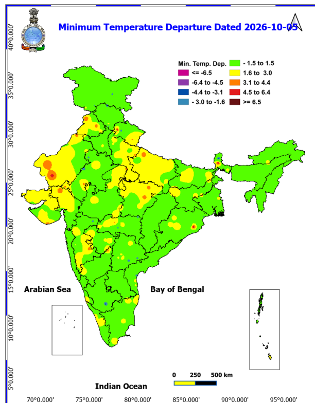
Fig. 4: Departure of Minimum Temp. Dated 2026-10-05
