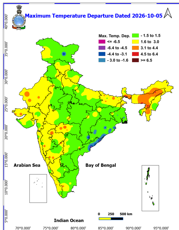
Fig. 2: Departure of Maximum Temp. Dated 2026-10-05
