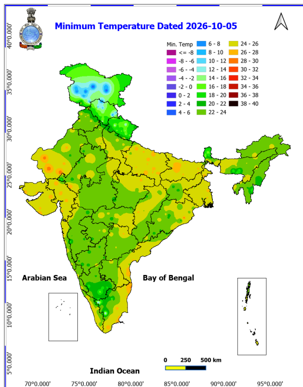
Fig. 3: Minimum Temperatures Dated 2026-10-05
