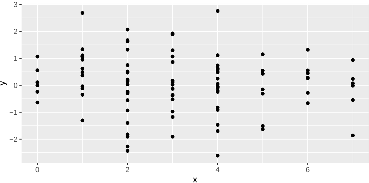
Scatterplot Diagram of X and Y
