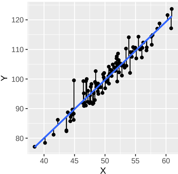
Homoscedastic Data
