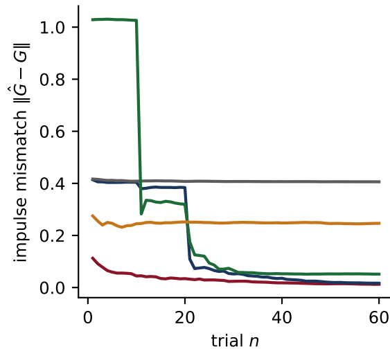
Model error vs true 3rd-order G
