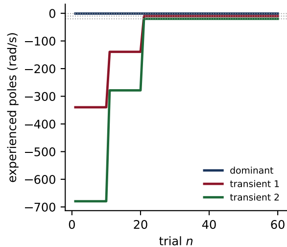
S2 pole locations
