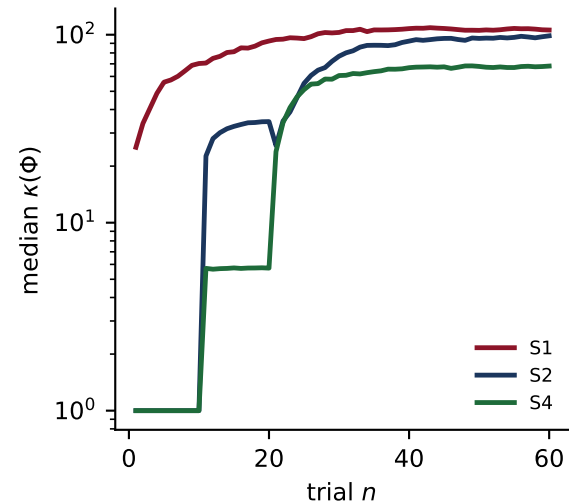
Hankel singular-value ratio
