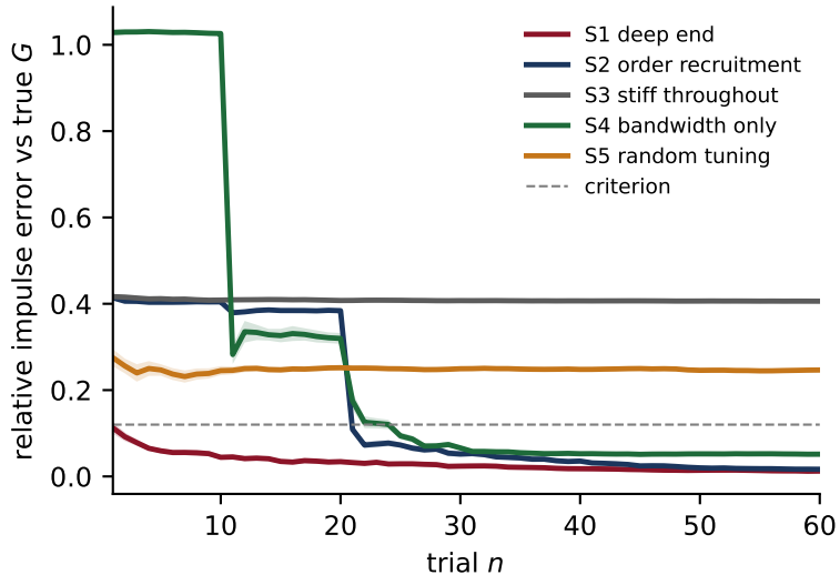
A Learning curves
