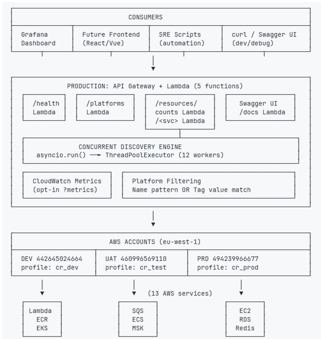
Figure 13: IA Resources Inventory API — Architecture Overview
