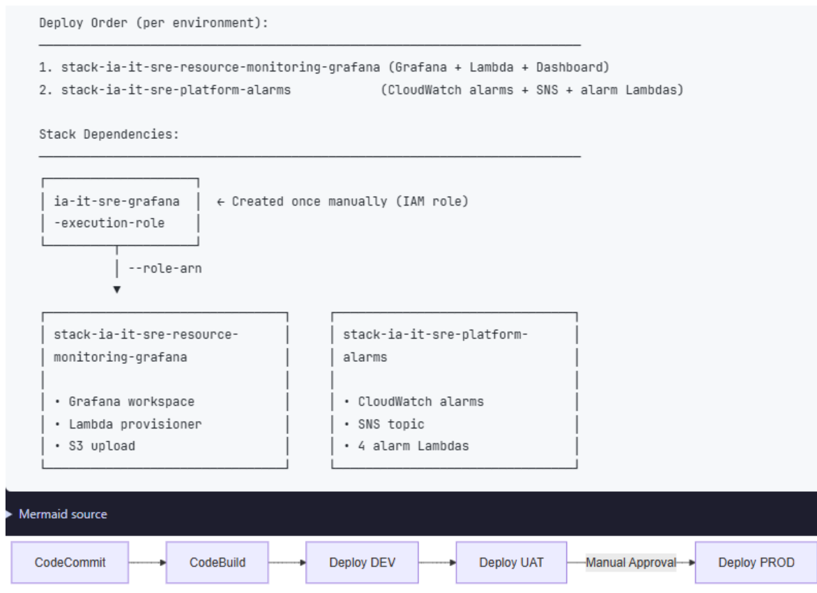
Figure 11: CI/CD Deployment Pipeline — CodeCommit to AMG Deployment Flow
