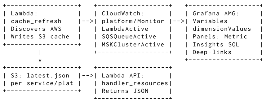
Figure 10.13: Inventory API — Grafana AMG Integration
