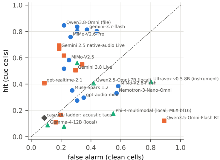
Probes: cue report rate
