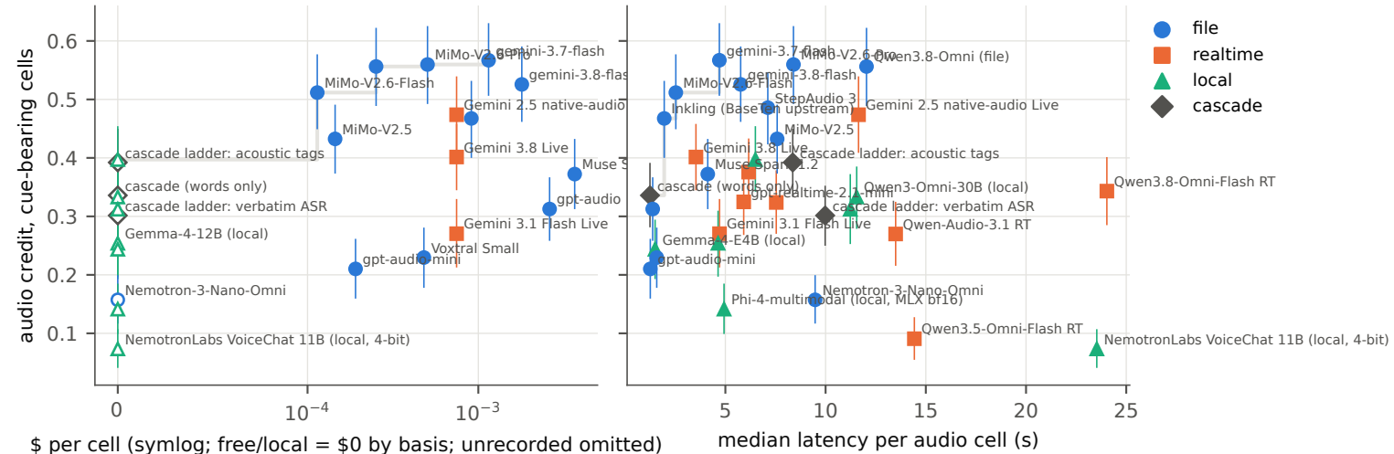
Cost and latency vs acting on the cue
