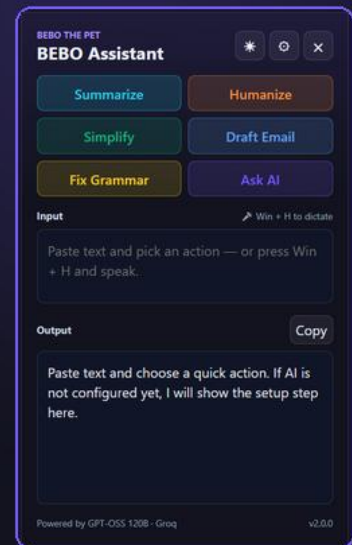
Real Panel UI (Ctrl+Shift+P)
