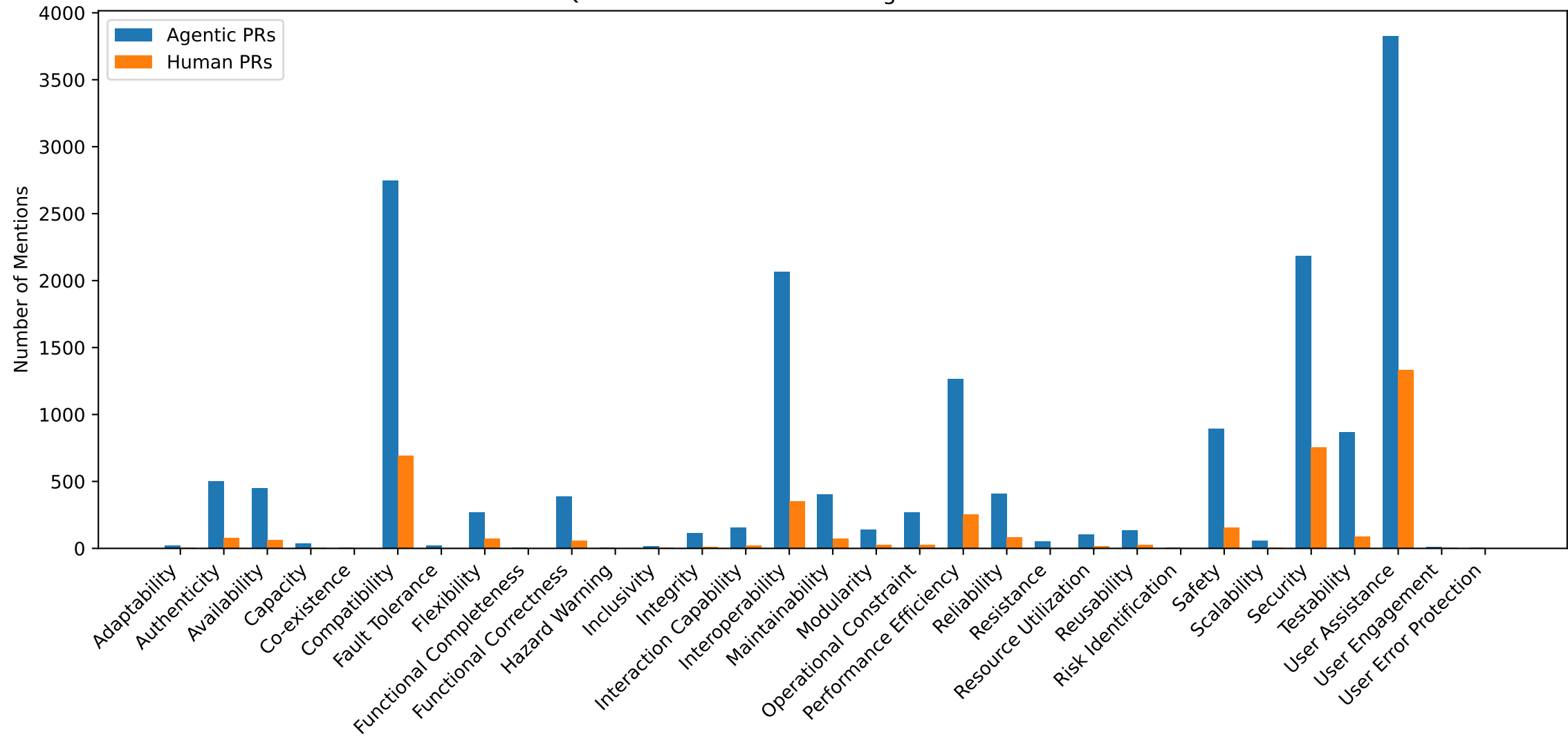
RQ1: ISO 25010 Mentions in Agentic vs Human PRs
