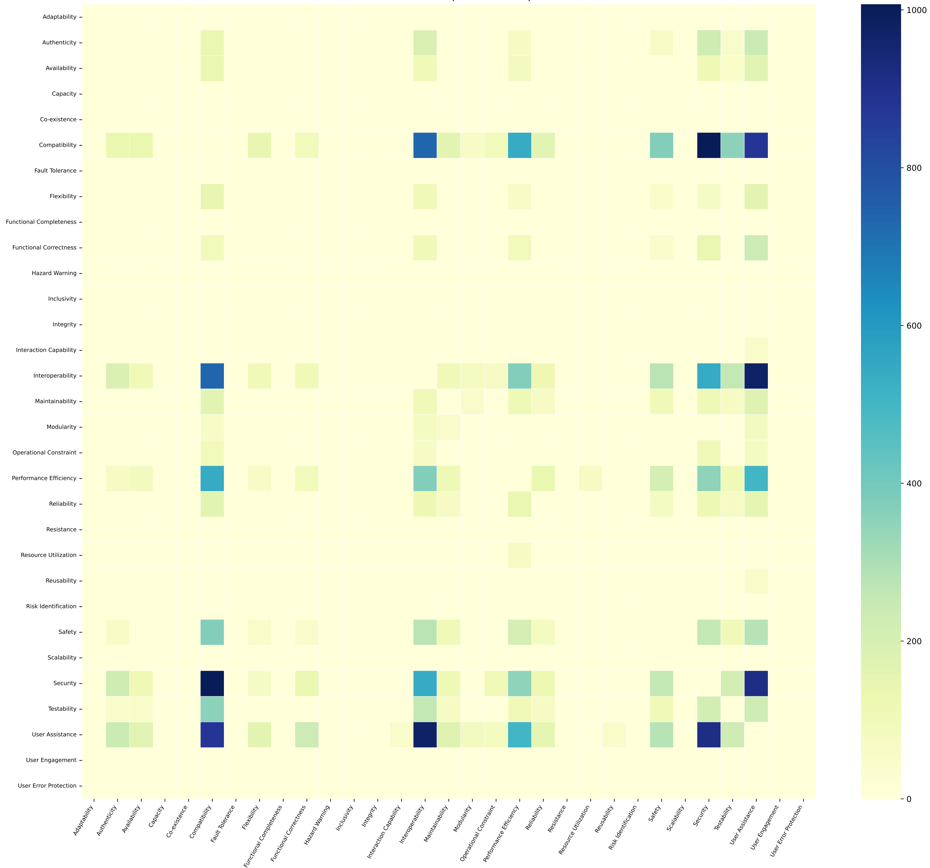
Co-occurrence (Filtered > 50)
