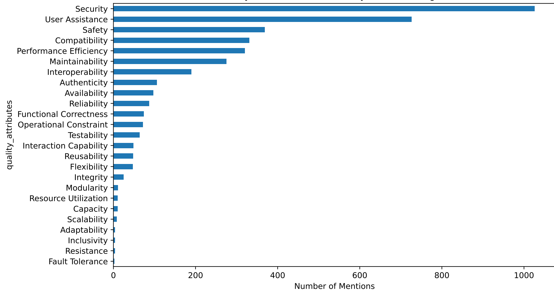
RQ3: Quality Attributes Discussed by Humans in Agentic PRs
