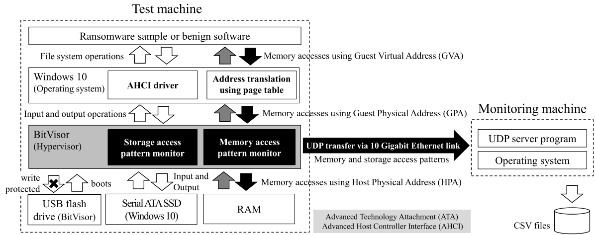
Fig. 2. Schematic diagram of thin hypervisor-based monitoring system to collect storage and memory access patterns.
