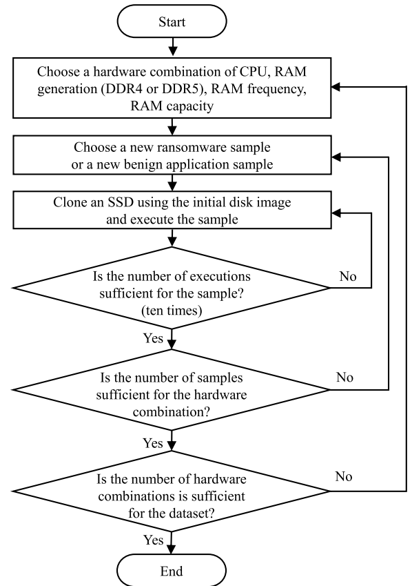
Fig. 3. Flow chart in creation of RanSMAP dataset.
