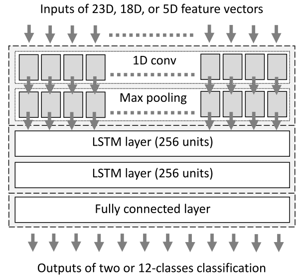
Fig. 5. Overview of our deep-learning-based ransomware detector consisting of a one-dimensional Convolutional Neural Network (1D-CNN) layer, a Max pooling layer, and two Long Short-Term Memory (LSTM) layers.
