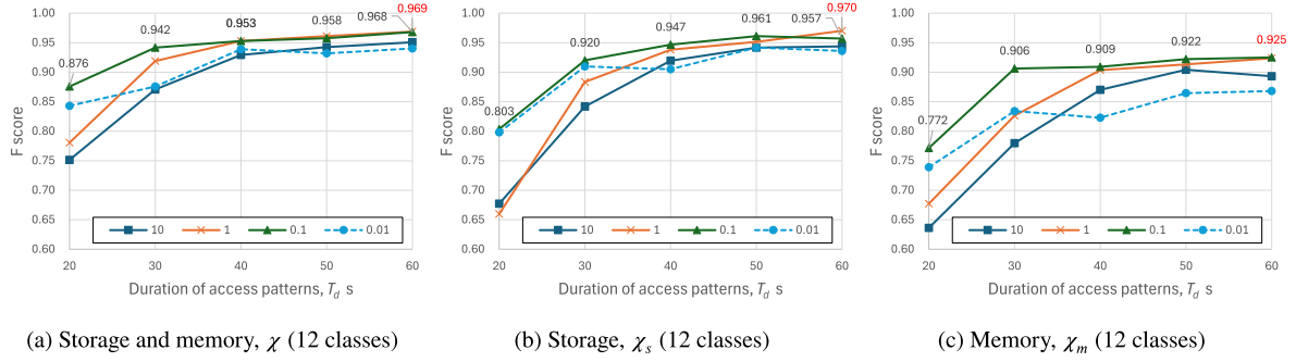
Fig. 8. Comparison of F scores in 12 classes by T_d = 20, 30, 40, 50 , and 60 s and T_{window} = 10, 1, 0.1 , and 0.01 s. The data labels are displayed only for T_{window} = 0.1 s except for the highest F score. (For interpretation of the references to color in this figure legend, the reader is referred to the web version of this article.)
