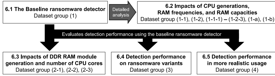
Fig. 6. The relationship between subsections of Section 6 and RanSMAP dataset groups. The dataset groups are shown in Tables 2 and 8.
