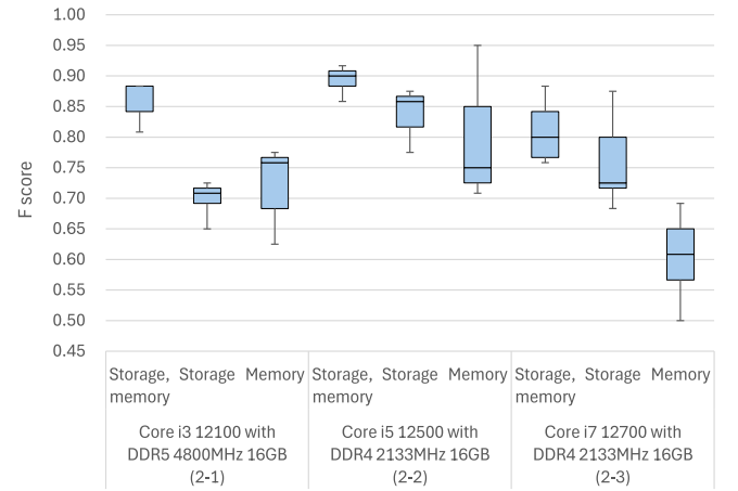
Fig. 13. Box plots of F scores of 12-classes classification when the baseline ransomware detectors predict a class of the access patterns of subgroup (2-1), (2-2), and (2-3); the baseline ransomware detector was trained using 100% of the group (1).
