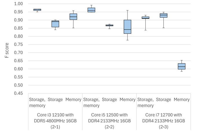
Fig. 12. Box plots of F scores of binary classification when the baseline ransomware detectors predict a class of the access patterns of subgroup (2-1), (2-2), and (2-3); the baseline ransomware detector was trained using 100% of the group (1).
