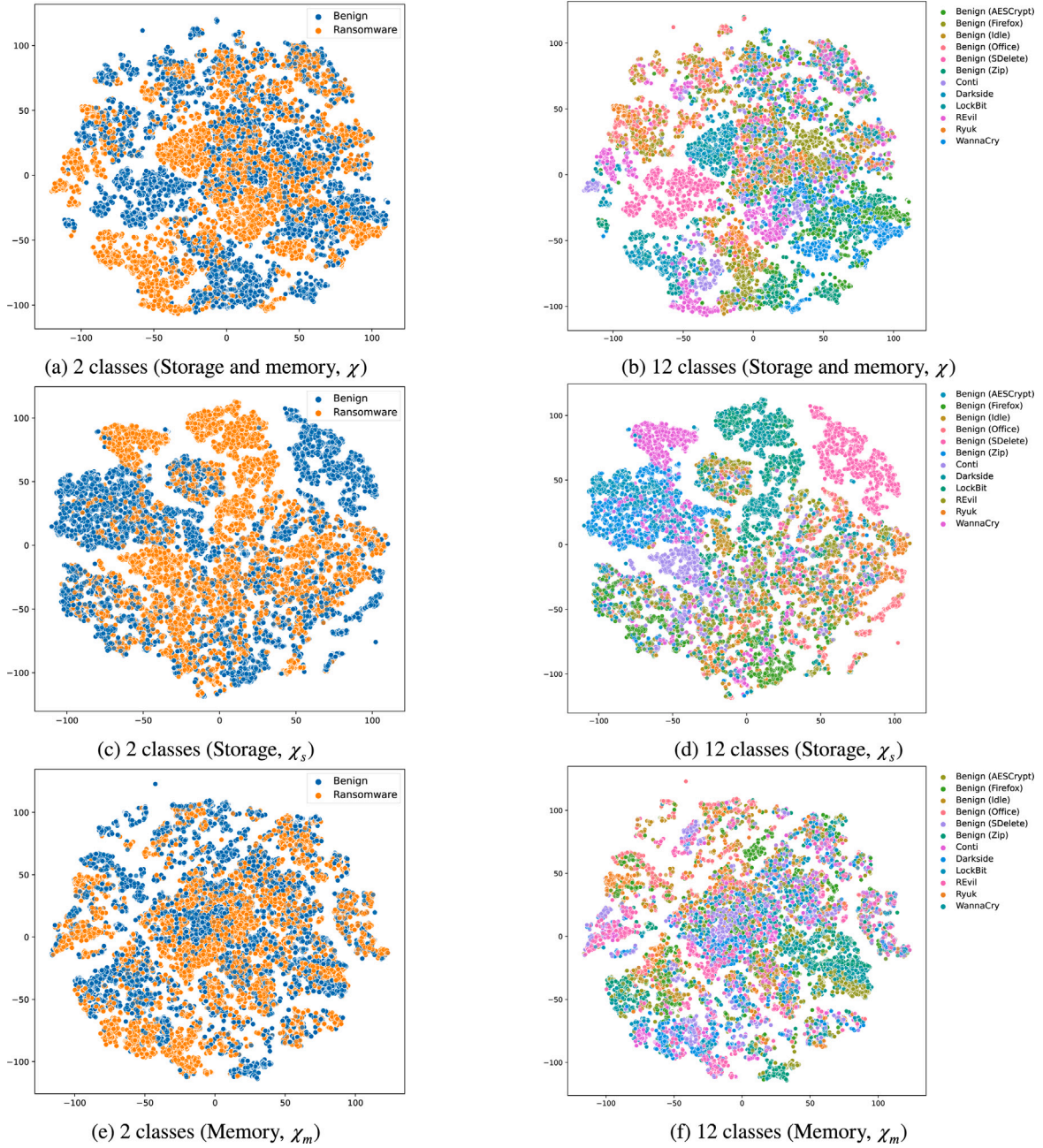
Fig. 4. Visualization by t-SNE ( T_{window} = 10 s and T_d = 30 s).
