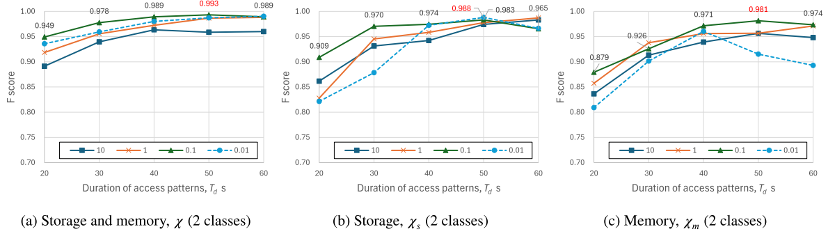
Fig. 7. Comparison of F scores in 2 classes by T_d = 20, 30, 40, 50, and 60 s and T_{window} = 10, 1, 0.1, and 0.01 s. The data labels are displayed only for T_{window} = 0.1 s, except for the highest F score in red. (For interpretation of the references to color in this figure legend, the reader is referred to the web version of this article.)
