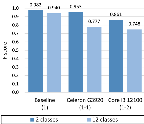
Fig. 10. F scores of the ransomware detectors trained using storage and memory features \chi excluding a CPU subgroup. The excluded subgroups are shown in horizontal axis titles, except for the baseline ransomware detector.
