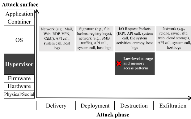
Fig. 1. Detection features of defense-in-depth ransomware detection systems in multiple attack phases and surfaces.
