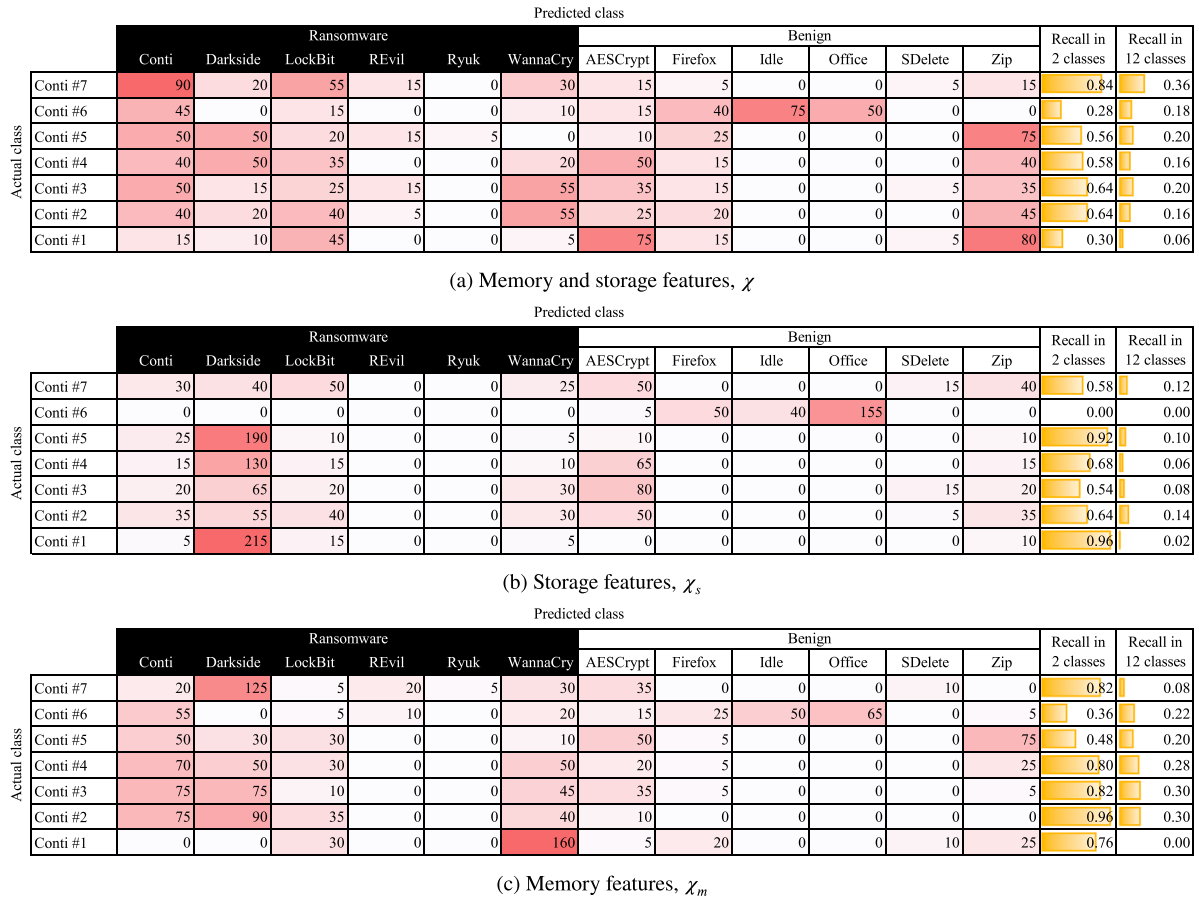
Fig. 14. Confusion matrices and recalls when the baseline ransomware detector predicts a class using the access patterns of the group (3), Conti ransomware variants. The baseline ransomware detector was trained using 100% of the group (1).
