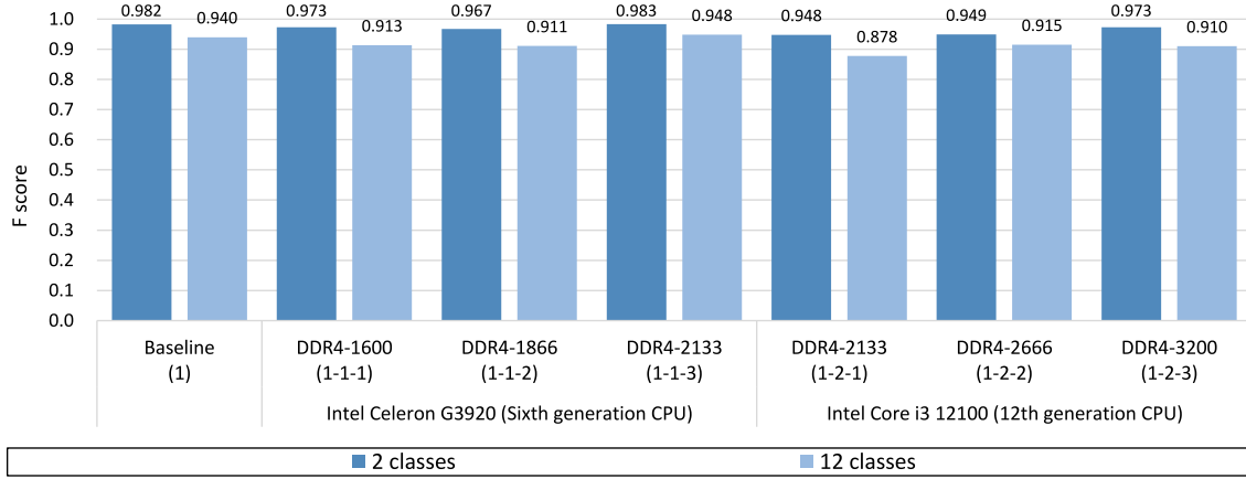
Fig. 9. F scores of the ransomware detectors trained using storage and memory features \chi excluding a RAM frequency subgroup. The excluded subgroups are shown in horizontal axis titles, except for the baseline ransomware detector.
