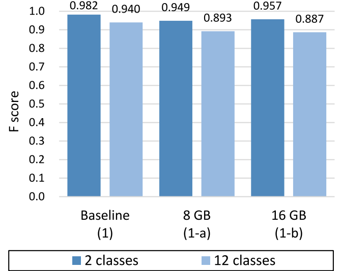
Fig. 11. F scores of the ransomware detectors trained using storage and memory features \chi excluding a RAM capacity subgroup. The excluded subgroups are shown in horizontal axis titles, except for the baseline ransomware detector.
