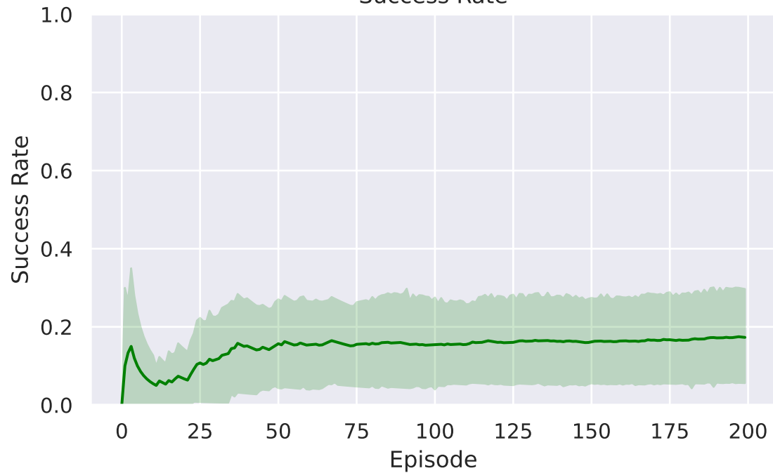
Success Rate
