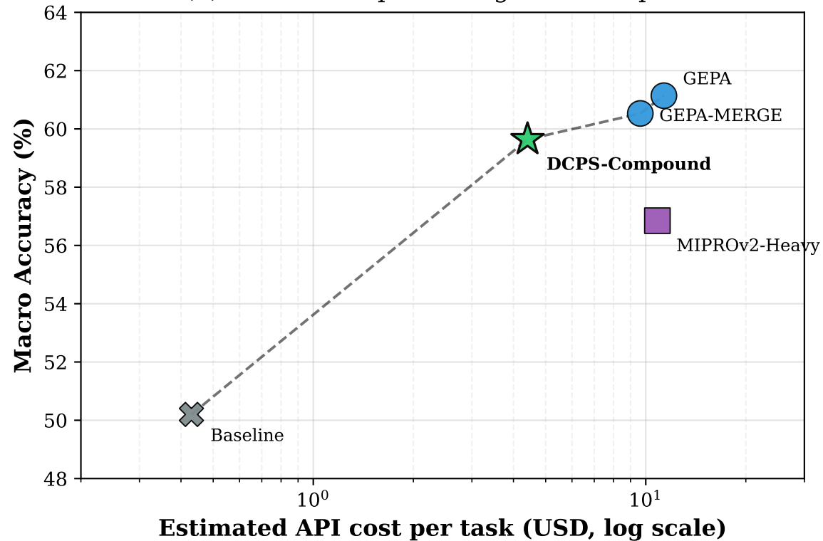
(b) Cost axis = price-weighted API spend
