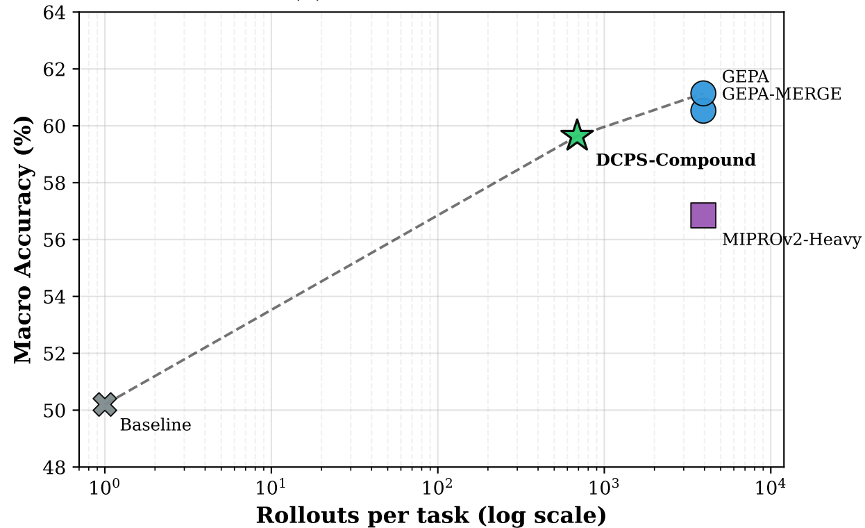
(a) Cost axis = rollouts
