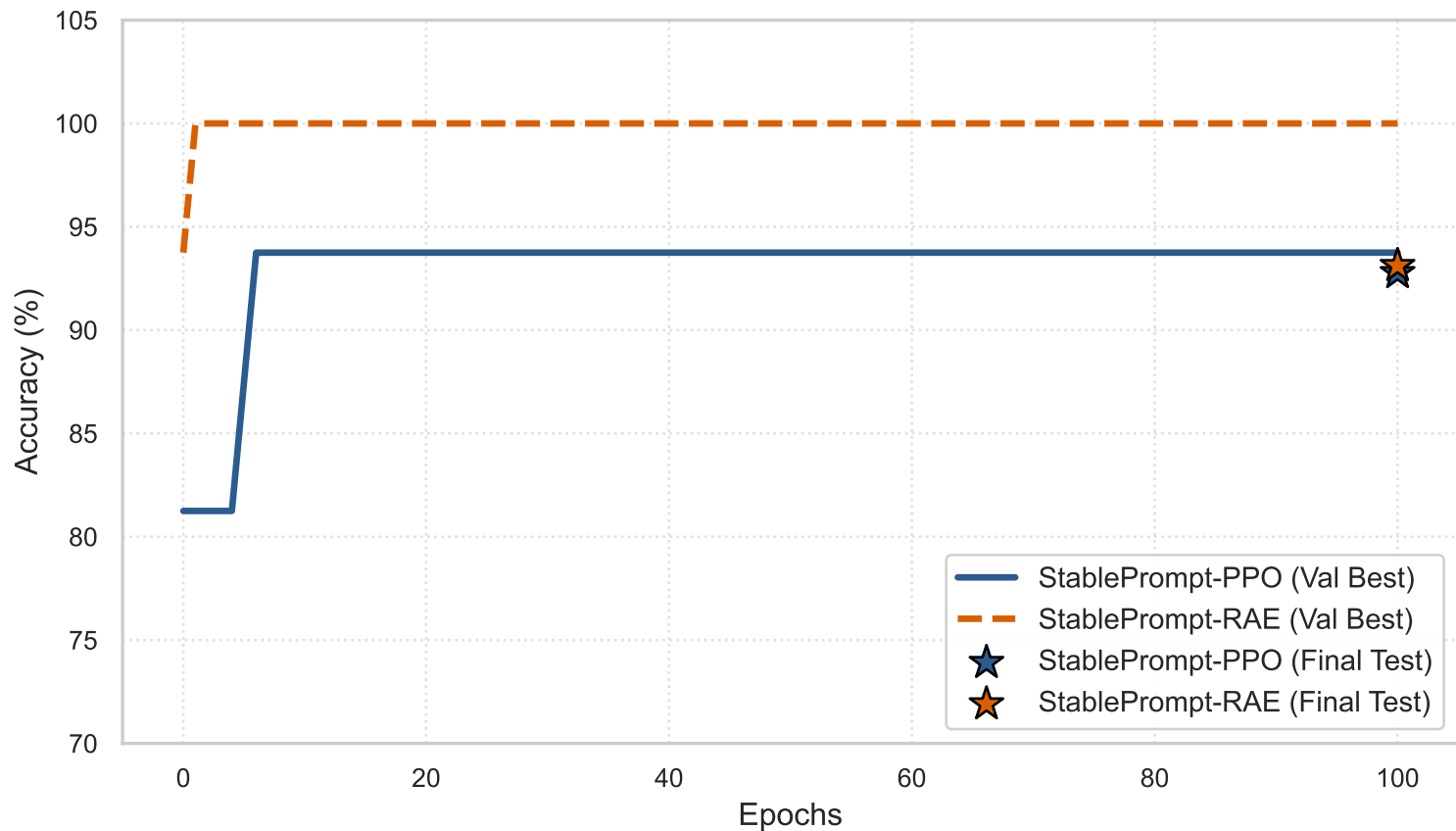
Gemma-1.1-7B-it on SST-2: StablePrompt-PPO vs StablePrompt-RAE (gr6jxsk8)
