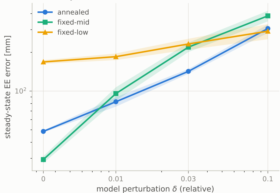
B steady-state error vs model error
