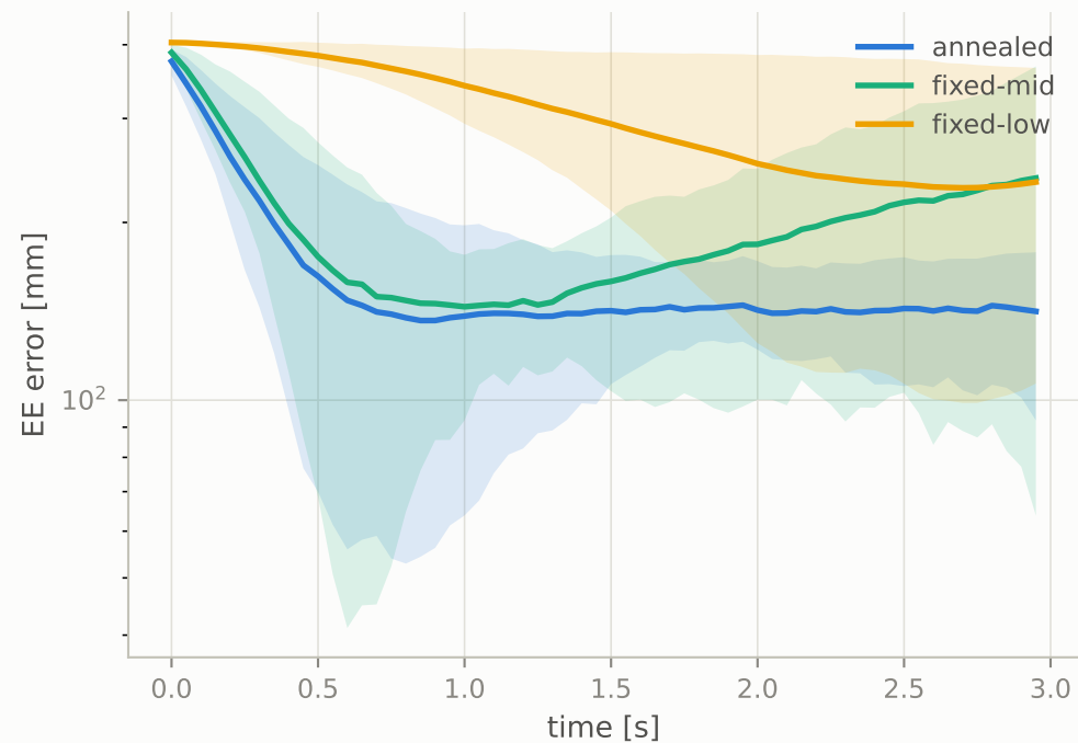
A closed-loop tracking, same model error ( \delta=0.03 )
