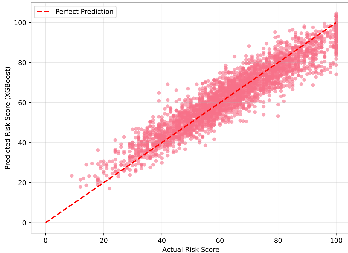
Risk Score Predictions
