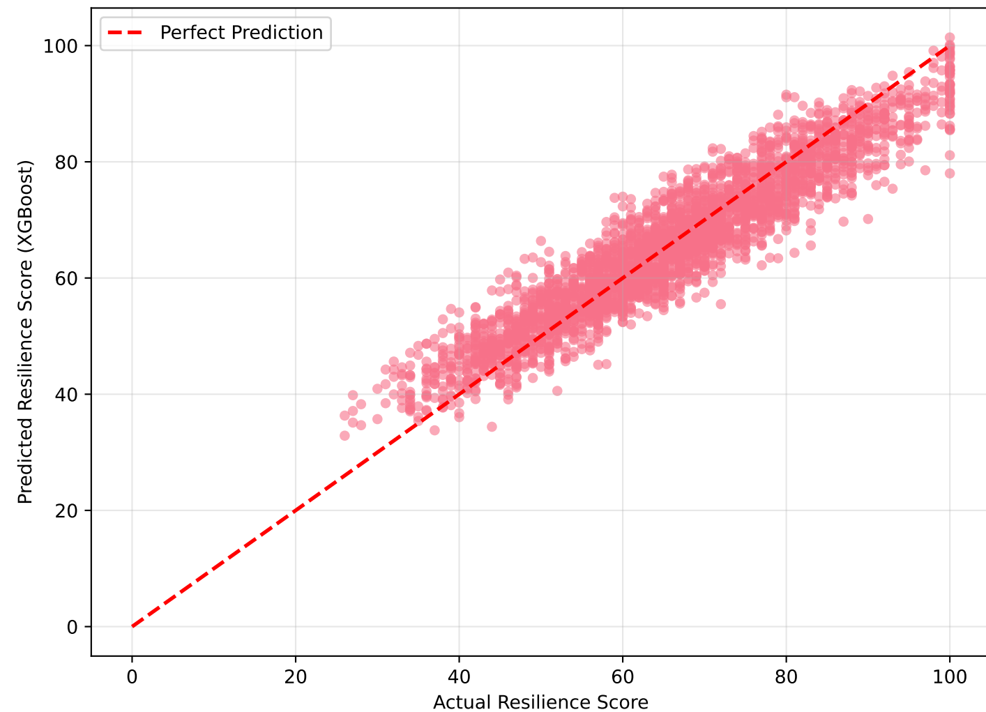
Resilience Score Predictions
