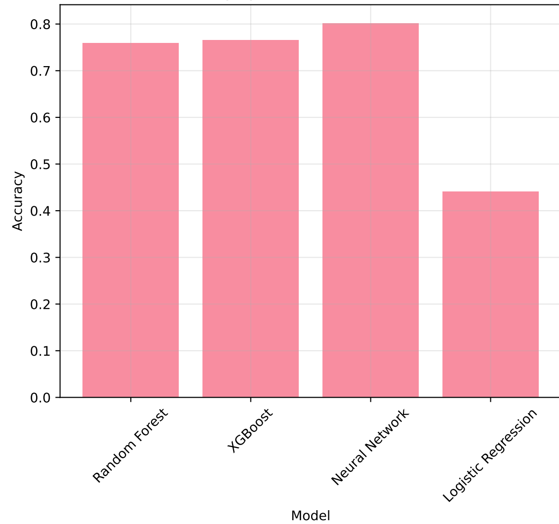
Risk Category Classification Performance
