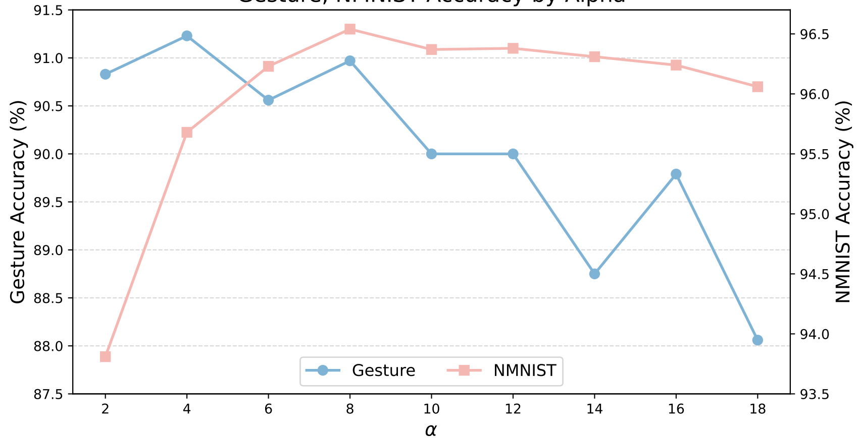
Gesture, NMNIST Accuracy by Alpha
