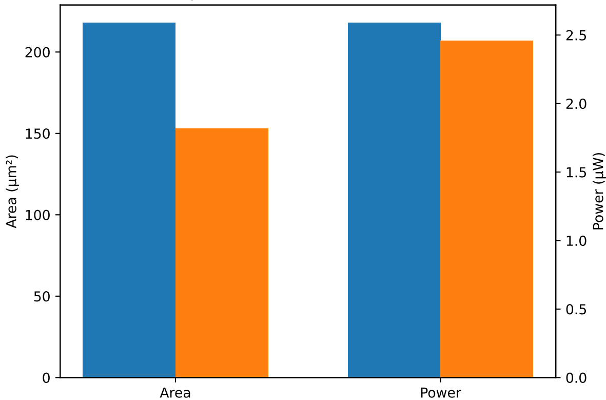
Synthesis Area and Running Power Post-Synthesis Simulation @ 1.0V, 20MHz
