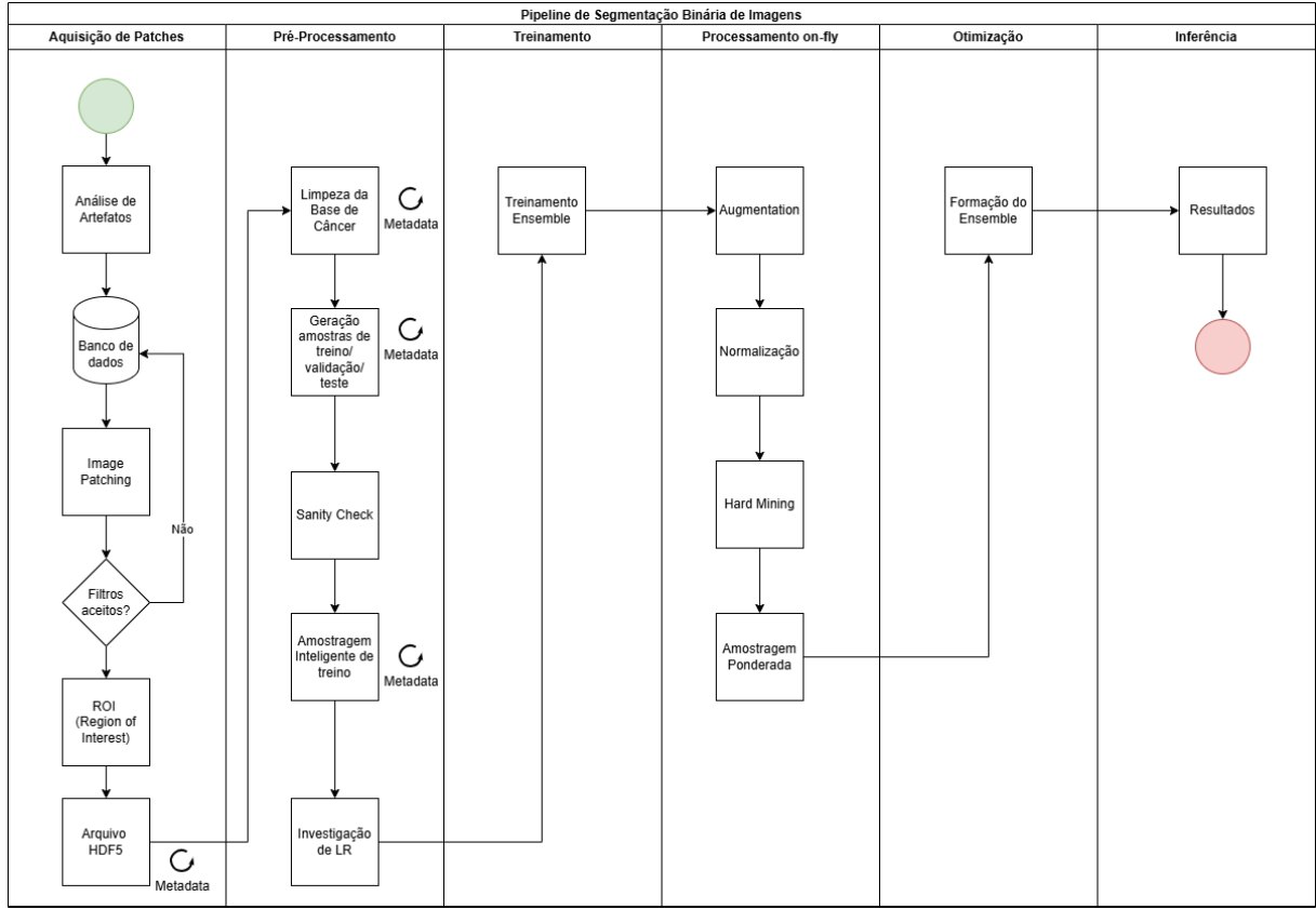
Figure 1: Overview of the implemented workflow. Whole-slide images and annotations are transformed into curated HDF5-backed patch datasets, split at the patient level, optionally reduced only in the training split, trained through a fixed model registry, combined by validation-only ensemble optimization, and evaluated with a frozen test-time recipe.
