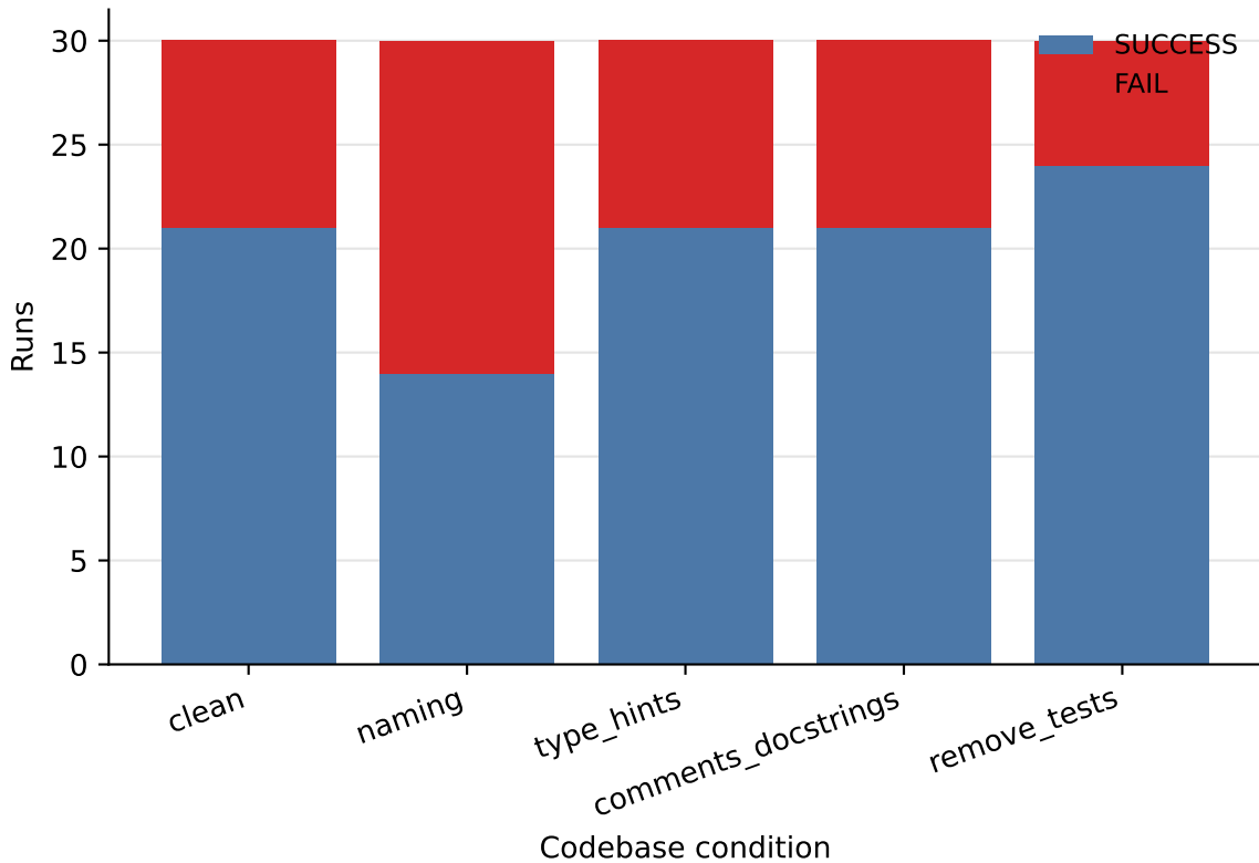
Solved And Failed Runs By Condition
