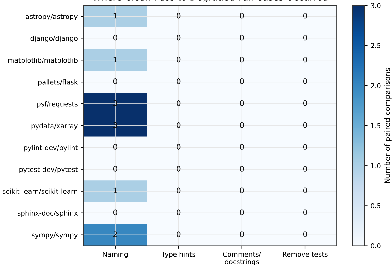
Where Clean-Pass to Degraded-Fail Cases Occurred
