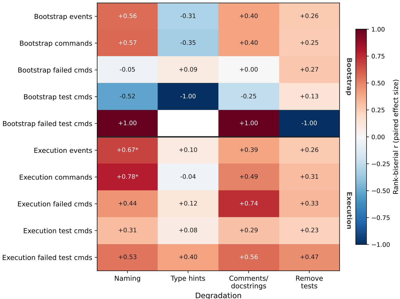
RQ2 effect size: each degradation × each phase metric Rank-biserial r from paired Wilcoxon (SWE-bench, 30-34 pairs/cond) Stars: Holm-adjusted *** p<0.001, ** p<0.01, * p<0.05
