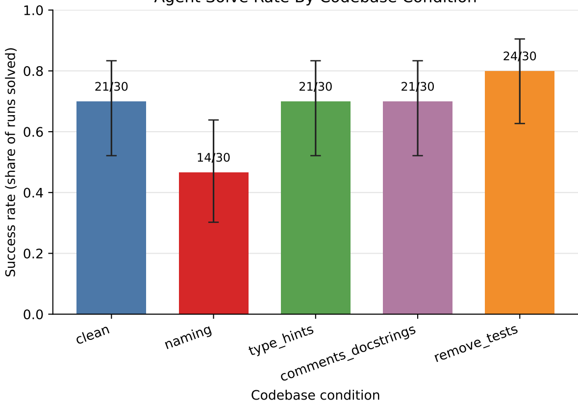
Agent Solve Rate By Codebase Condition
