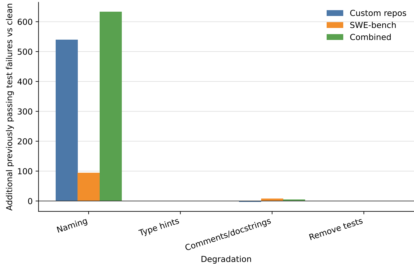
Naming Carries The Largest Regression Burden
