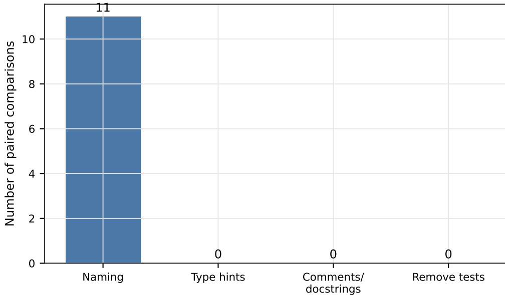
Cases Where Clean Passed but Degraded Failed
