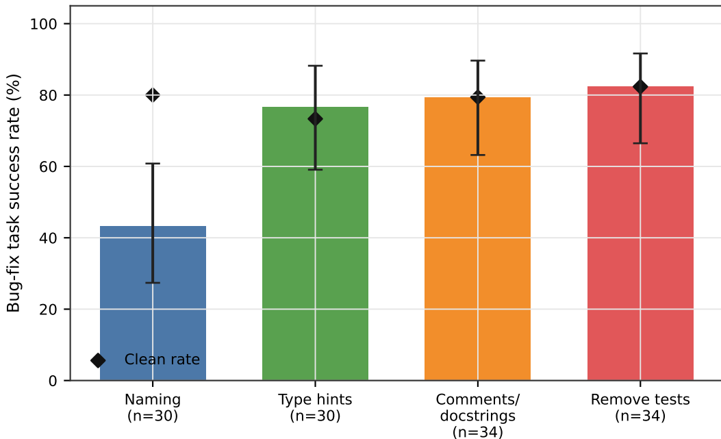
How Often Codex Solved the Task After Each Degradation
