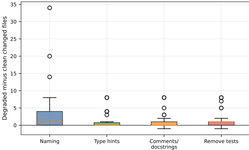
How Many More or Fewer Files Codex Changed
