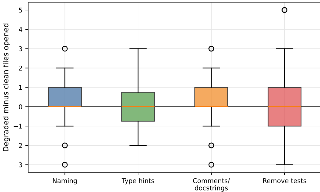
Early File Exploration Before the First Edit
