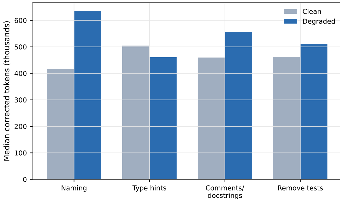
Typical Token Use in Clean vs Degraded Runs
