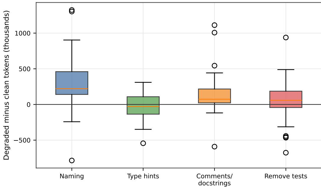
Extra or Fewer Tokens Used After Degradation
