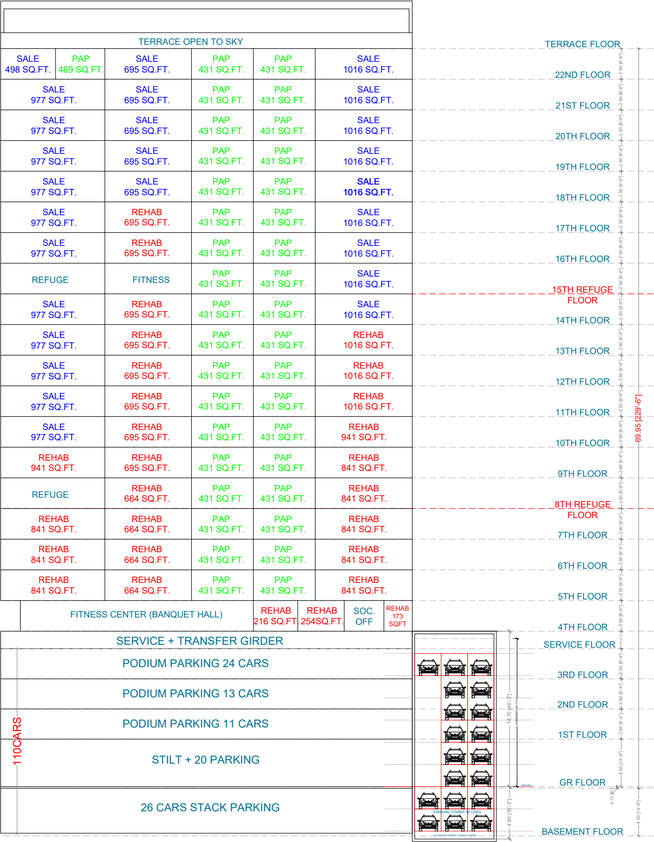
SCHEMATIC SECTION
