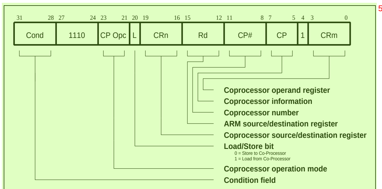
Figure 4-27: Coprocessor register transfer instructions 6
