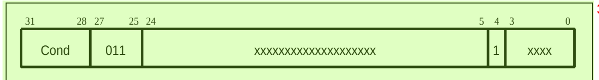
Figure 4-28: Undefined instruction 4
