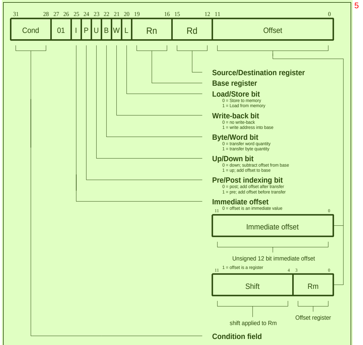
Figure 4-14: Single data transfer instructions 6
