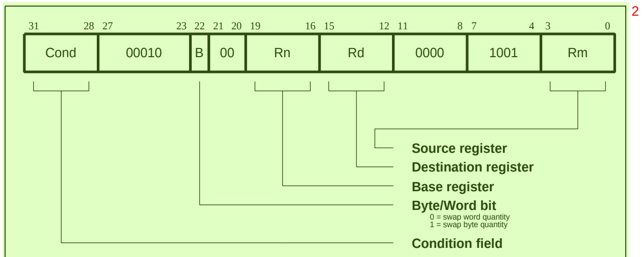
Figure 4-23: Swap instruction 3
