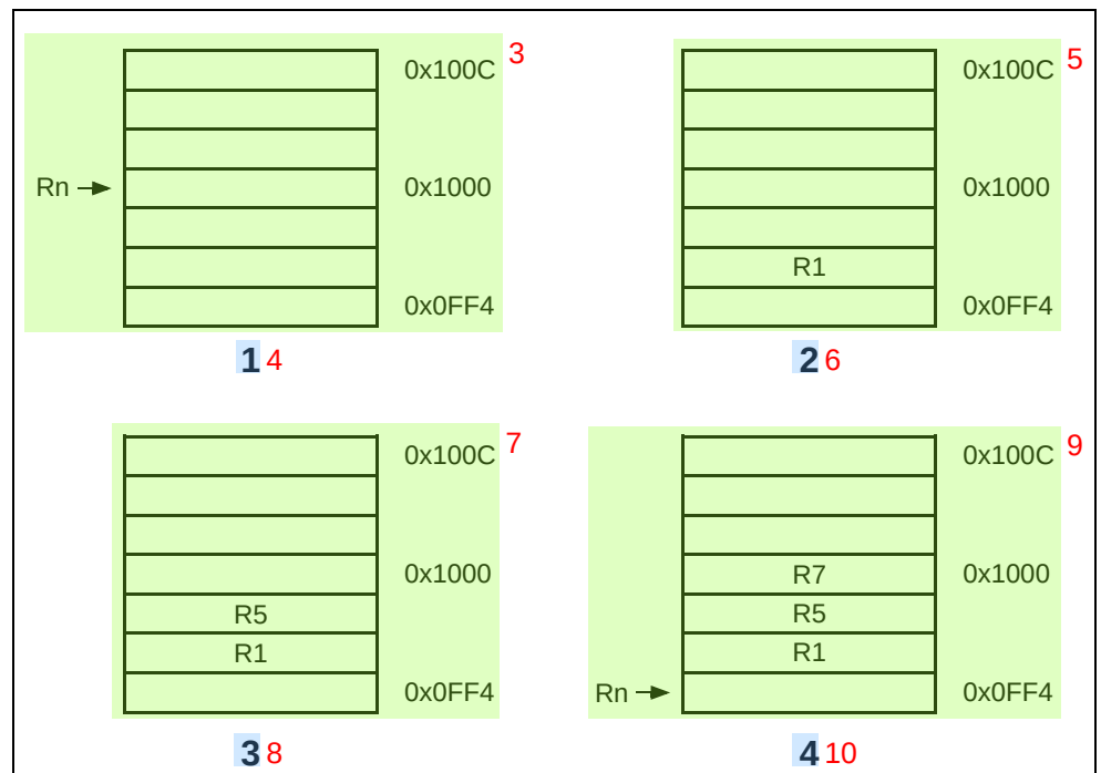
Figure 4-21: Post-decrement addressing
