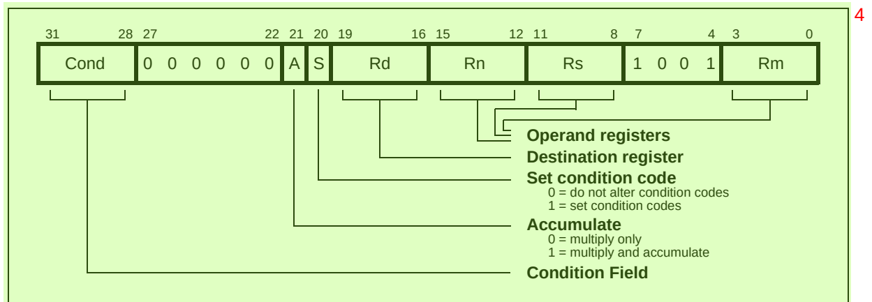
Figure 4-12: Multiply instructions 5
