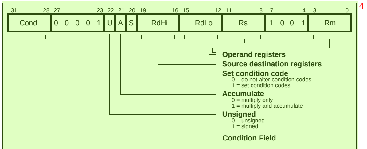
Figure 4-13: Multiply long instructions 5
