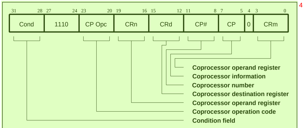
Figure 4-25: Coprocessor data operation instruction 5
