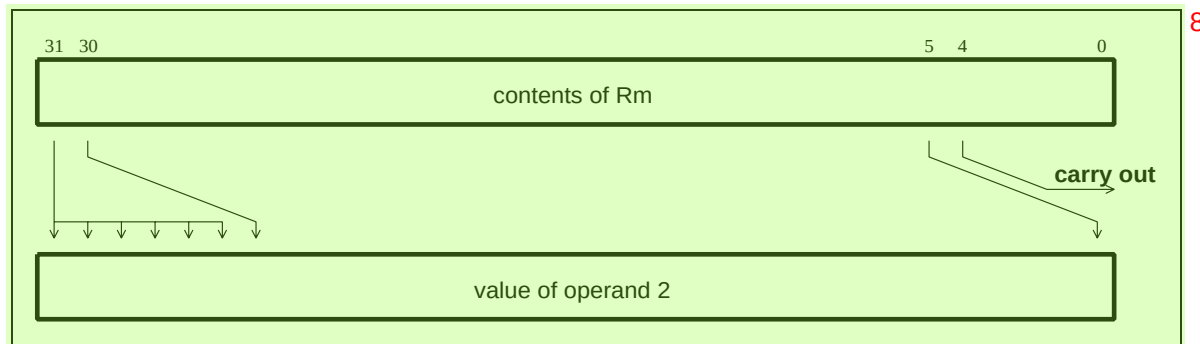
Figure 4-8: Arithmetic shift right 9
