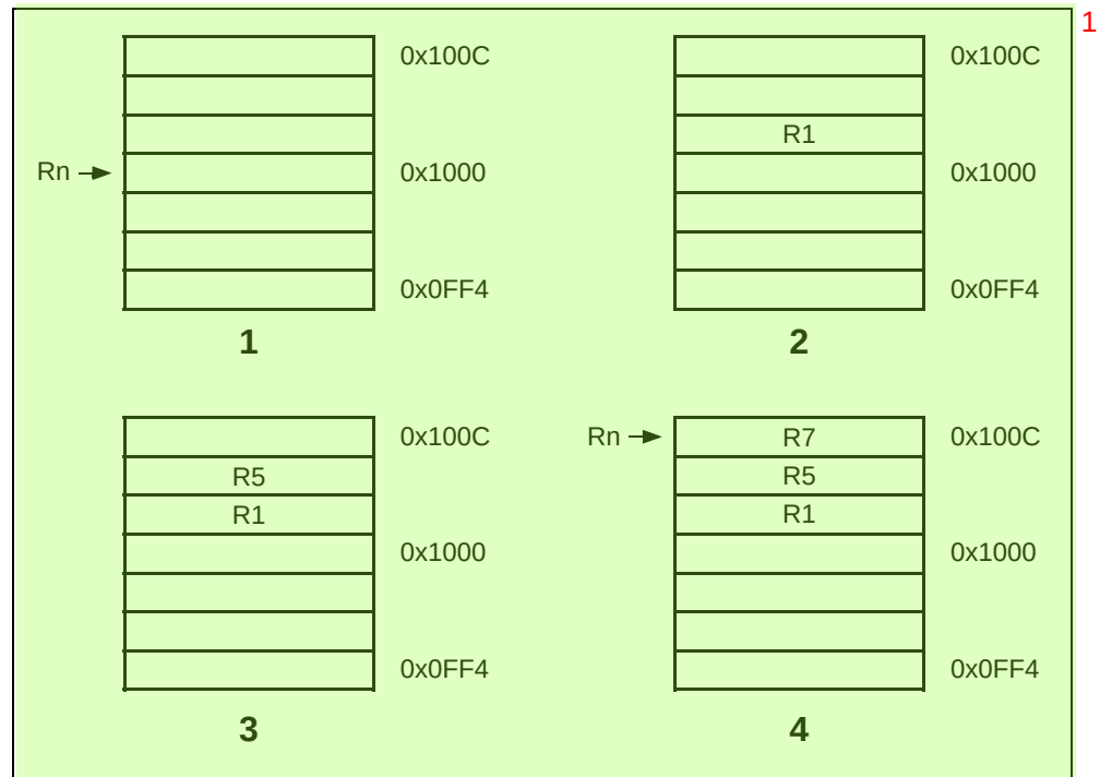
Figure 4-20: Pre-increment addressing
