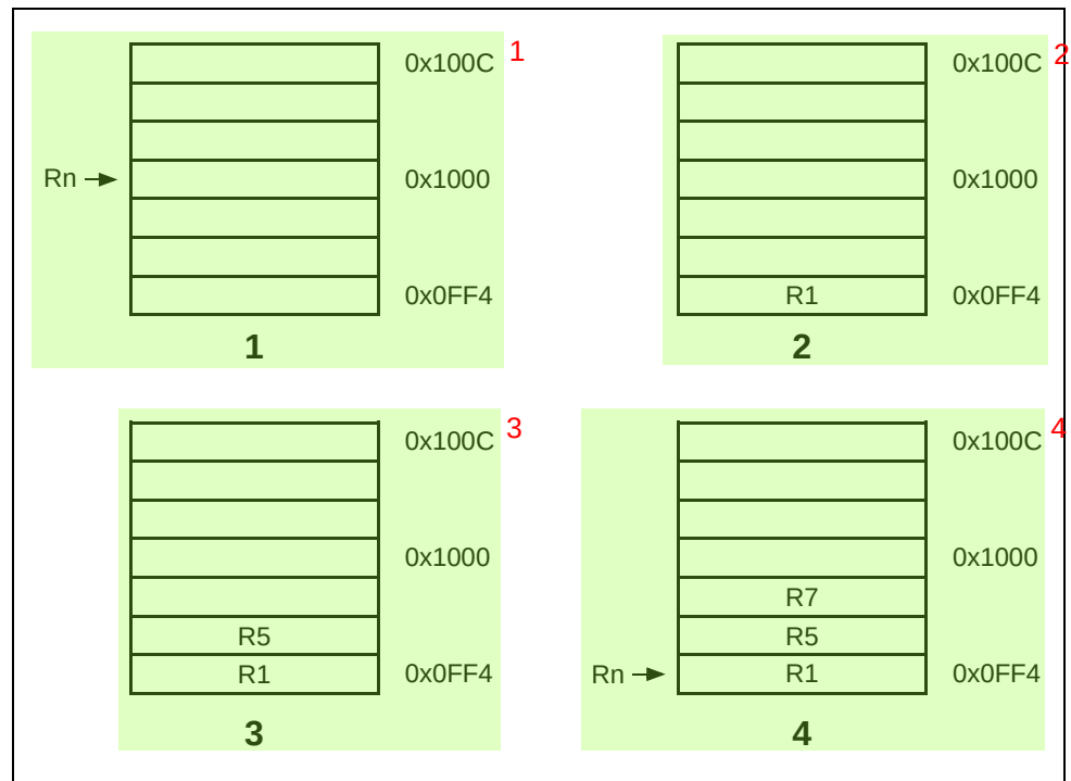
Figure 4-22: Pre-decrement addressing
