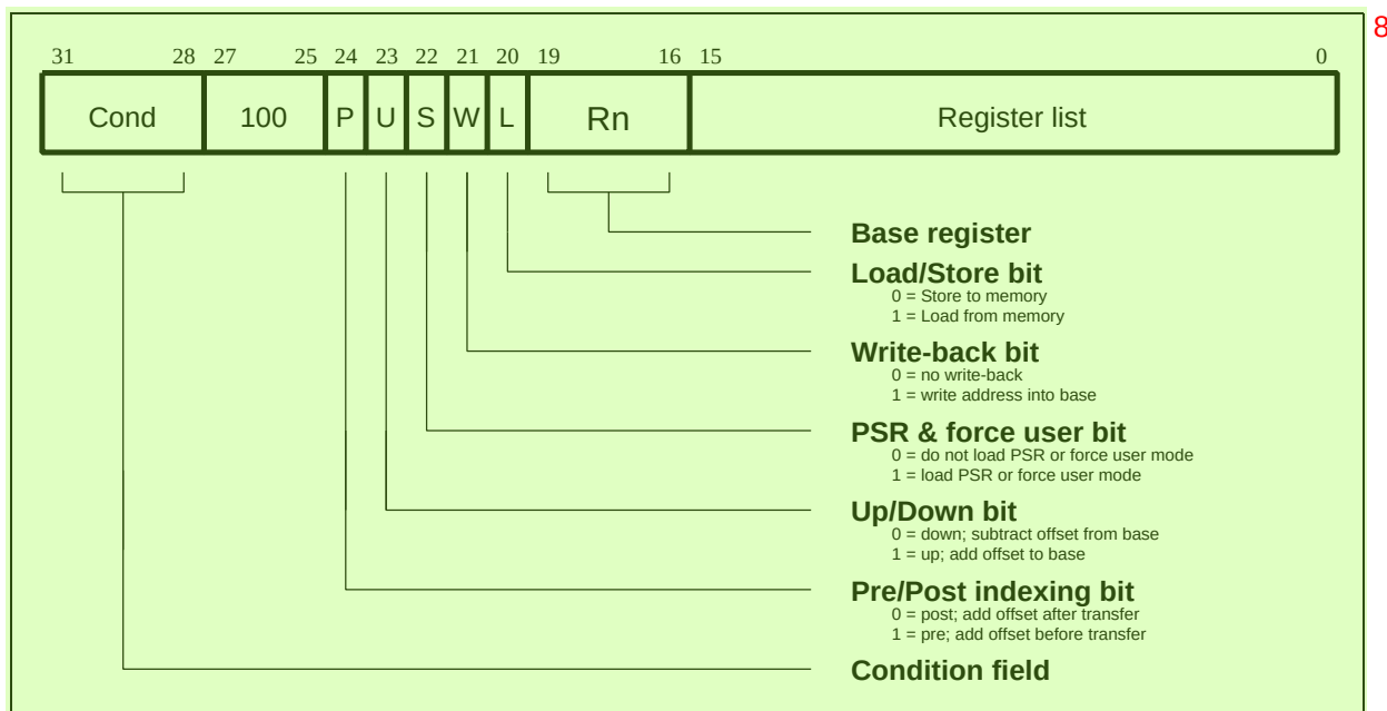
Figure 4-18: Block data transfer instructions 8
