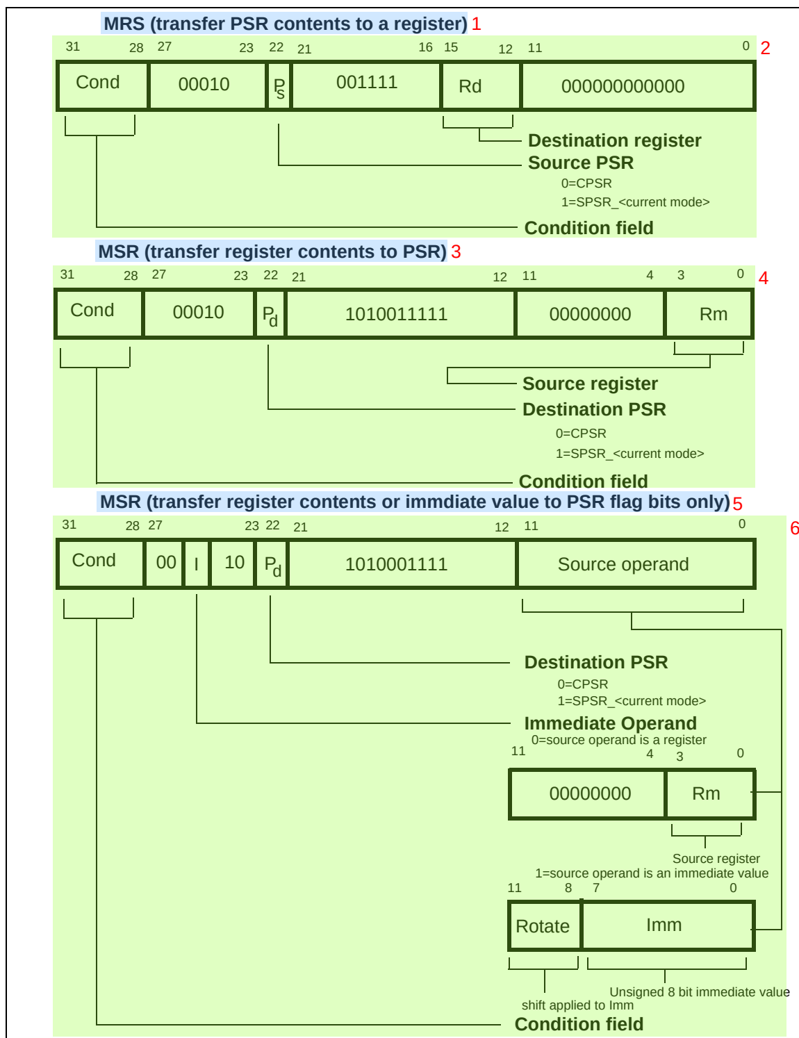
Figure 4-11: PSR transfer 7
