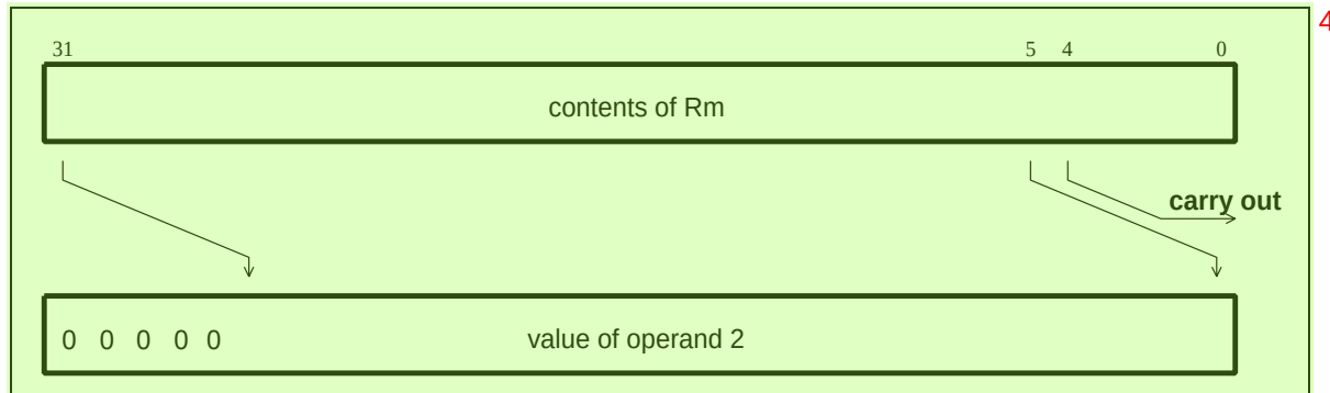
Figure 4-7: Logical shift right 5
