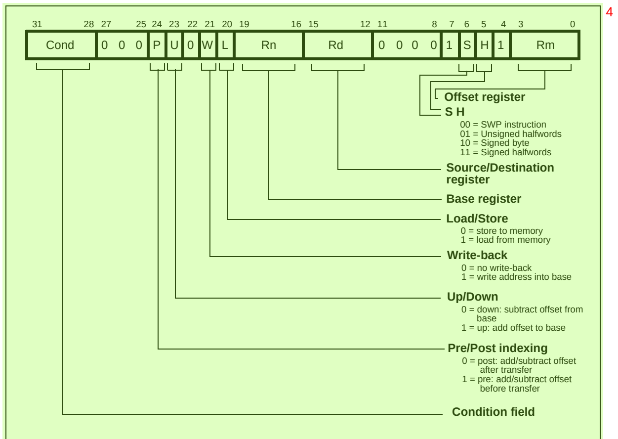
Figure 4-16: Halfword and signed data transfer with register offset 5
