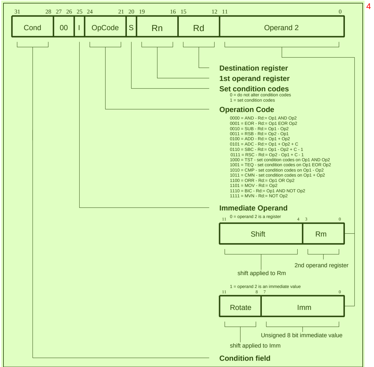
Figure 4-4: Data processing instructions 5
