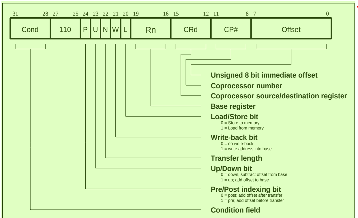
Figure 4-26: Coprocessor data transfer instructions 5
