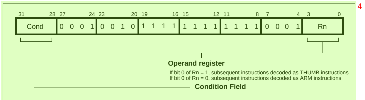
Figure 4-2: Branch and Exchange instructions 5
