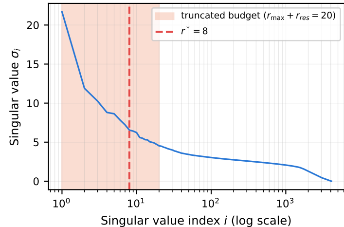
(a) Raw spectrum, layer-0 q_proj ( d = 4096 )
